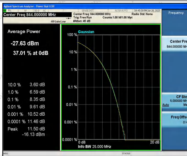
Band26-15MHz-QPSK-26765-1RB#0
