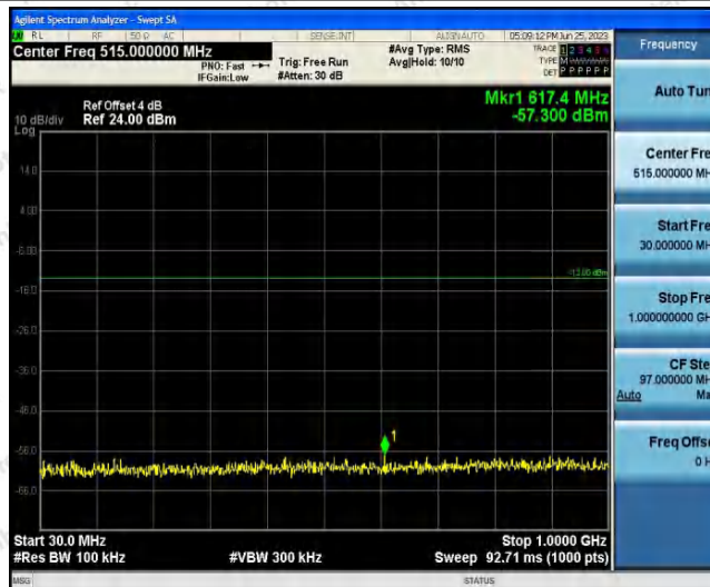
Band25-1.4MHz-QPSK-26365-1RB#0-Range1:30~1000MHz
