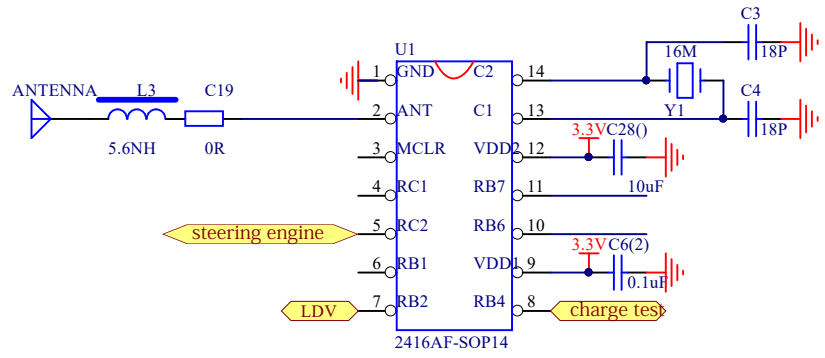
PAN2416AF-SOP14
