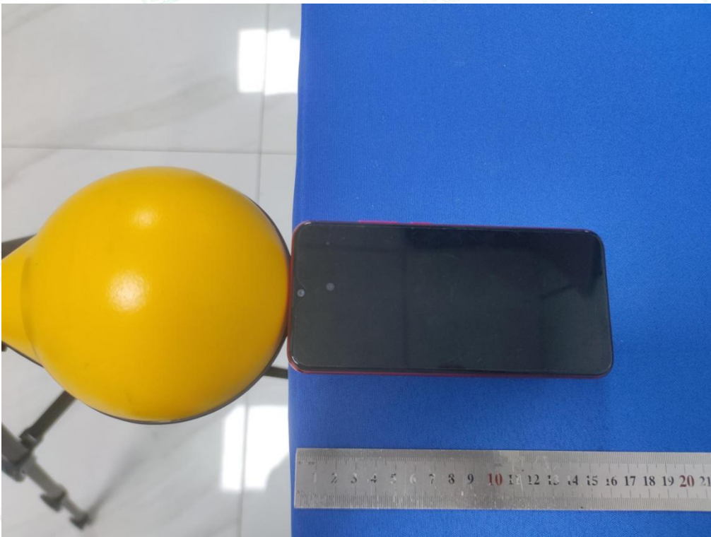
Test Position D(0cm) - Exposure photo from side edge surface-Front(TM1)
