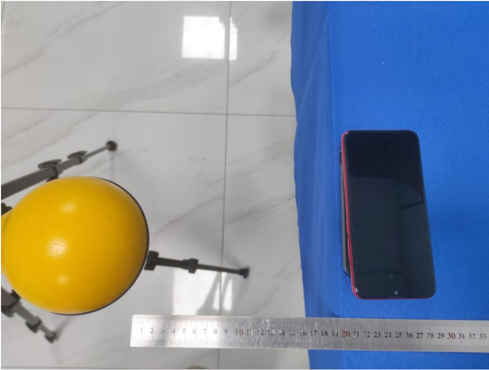
Test Position E(20cm) - Exposure photo from side edge surface-Right(TM1)
