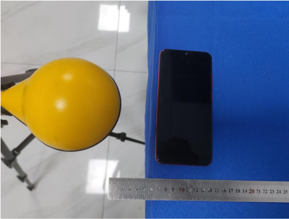
Test Position C(6cm) - Exposure photo from side edge surface-Left(TM1)
