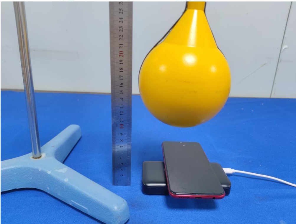
Test Position A (15cm) - Exposure photo from top surface (TM1)
