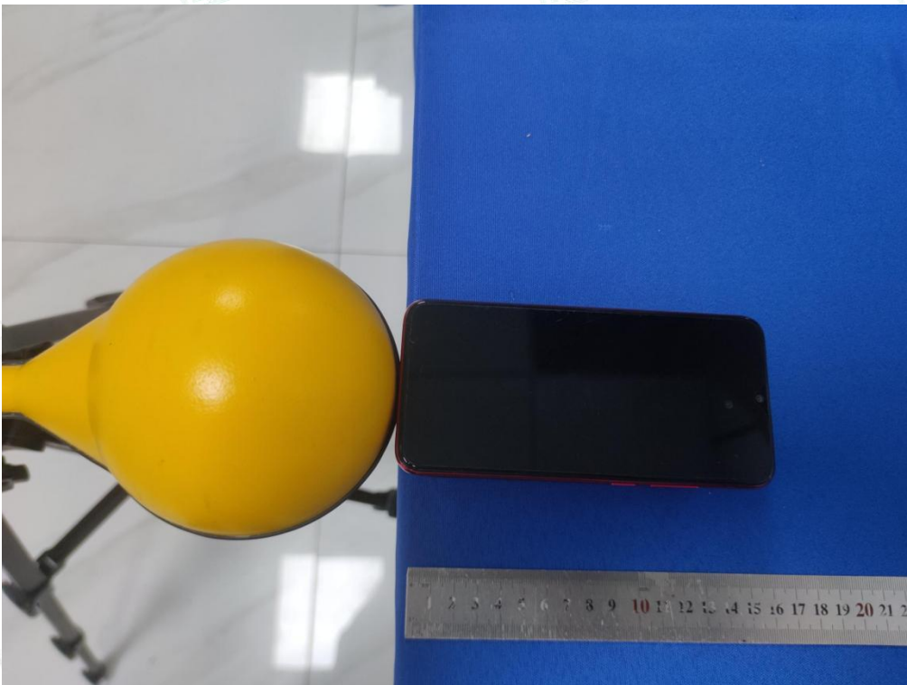
Test Position B(0cm) - Exposure photo from side edge surface-Rear(TM1)
