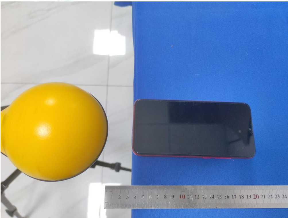
Test Position B(4cm) - Exposure photo from side edge surface-Rear(TM1)
