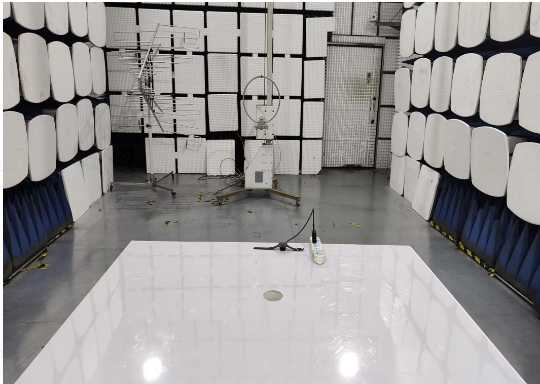
Radiated Emission below 30MHz-AC adapter charge mode
