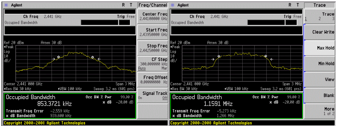
GFSK Middle channel
