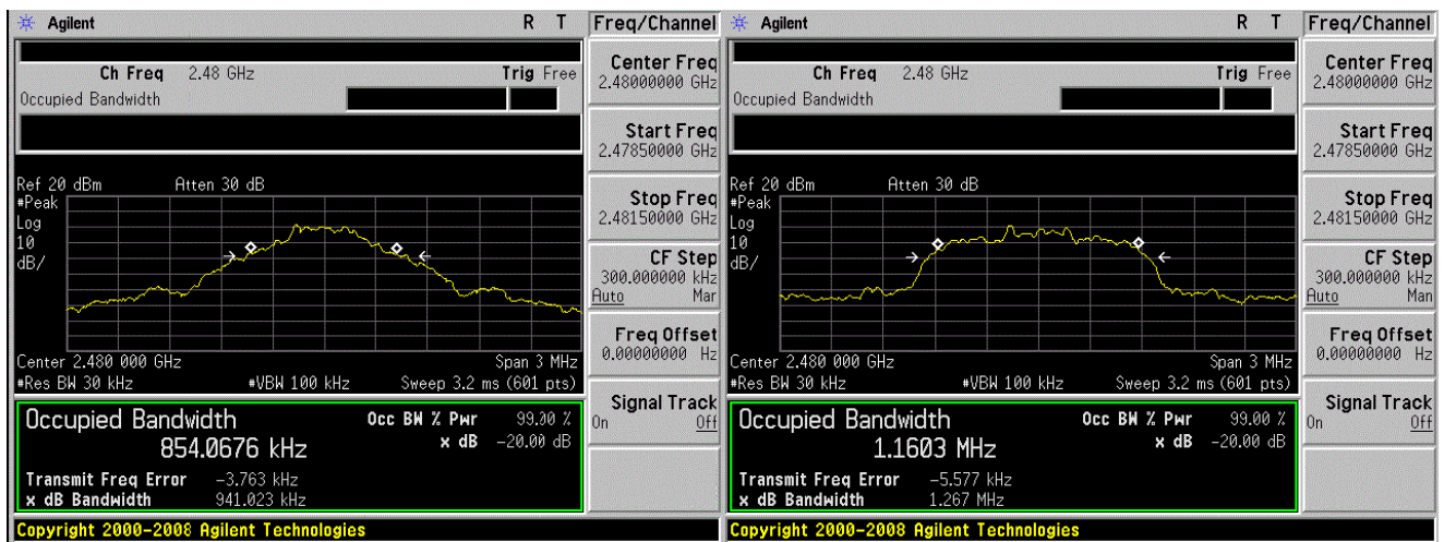
GFSK Highest channel
