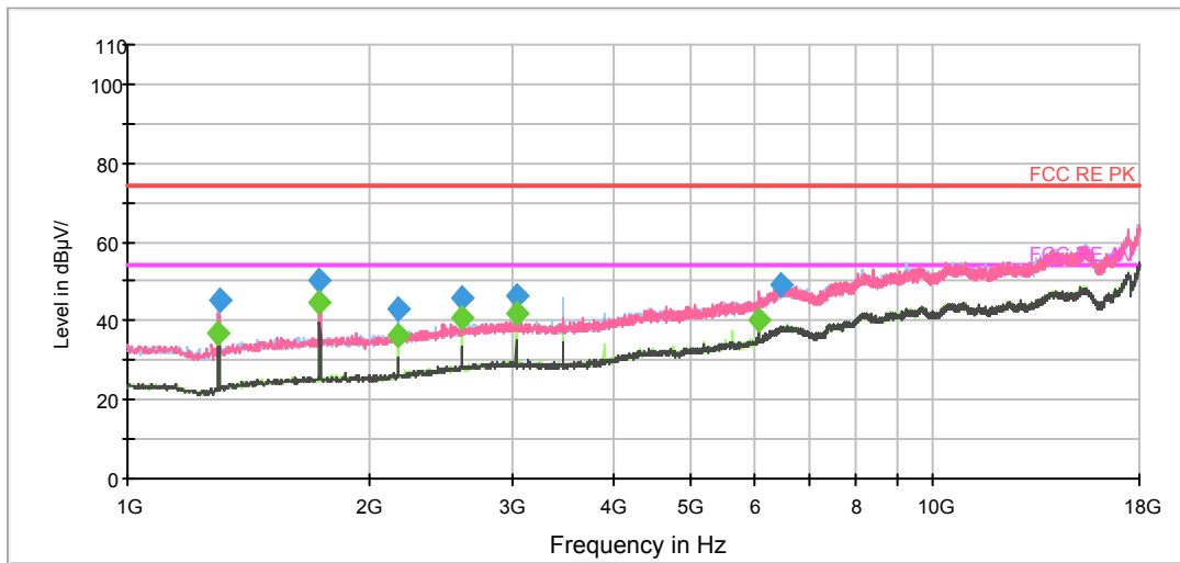
Radiates Emission from 1GHz to 18GHz
