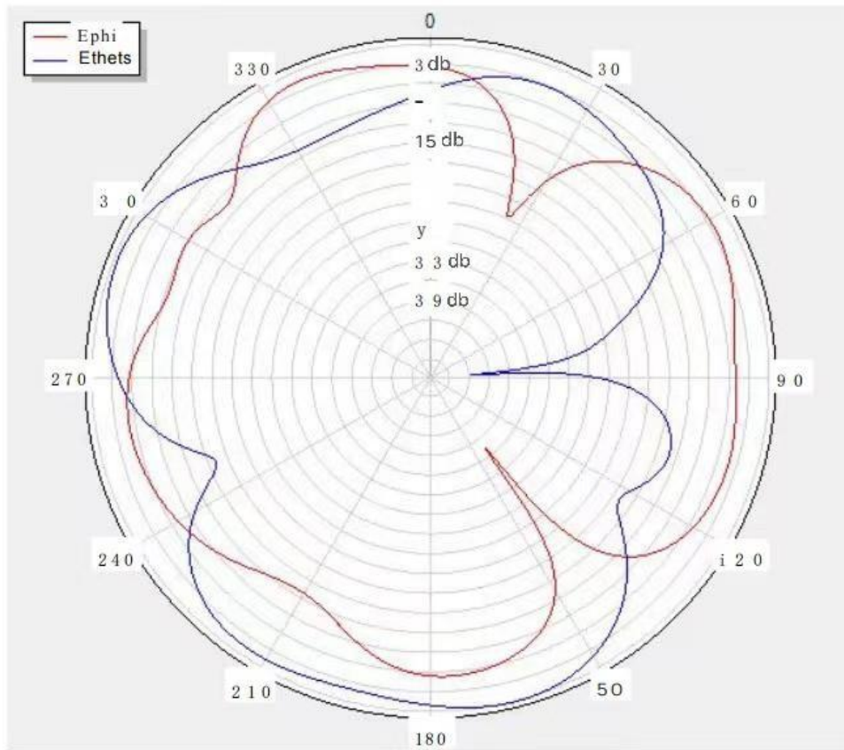
Theta=90 freq=2490MHz
