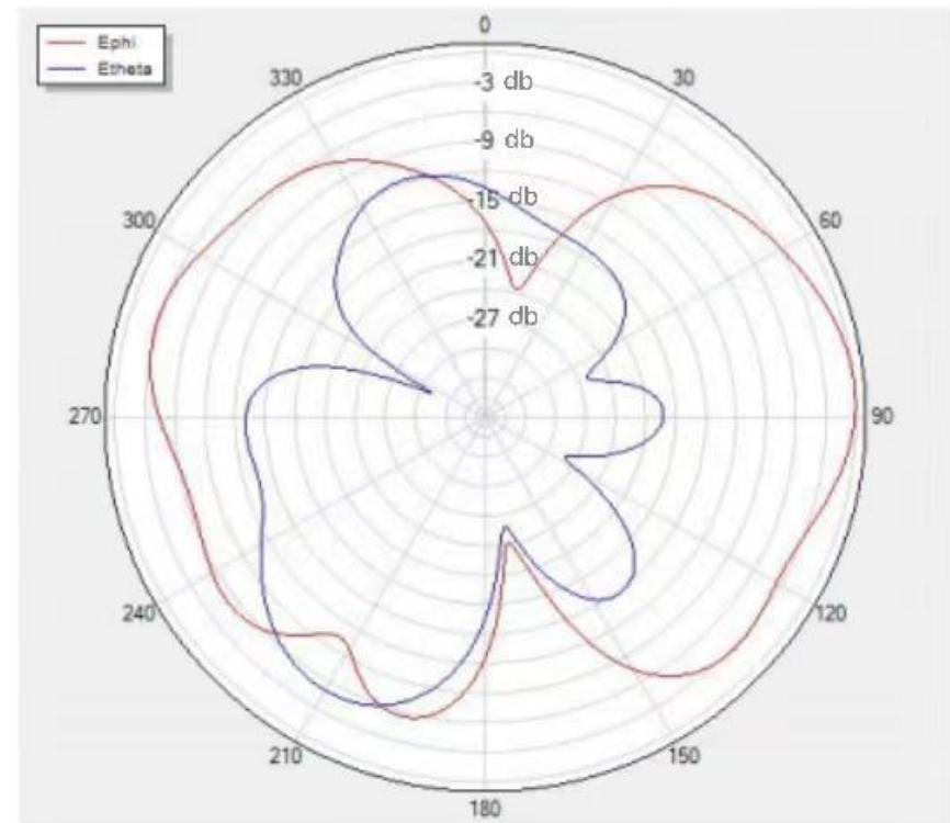
Phi=90 freq=2450MHz
