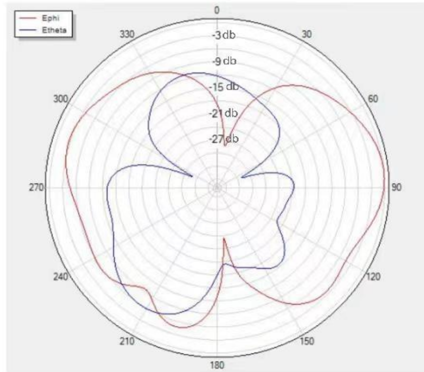
Phi=90 freq=2500MHz
