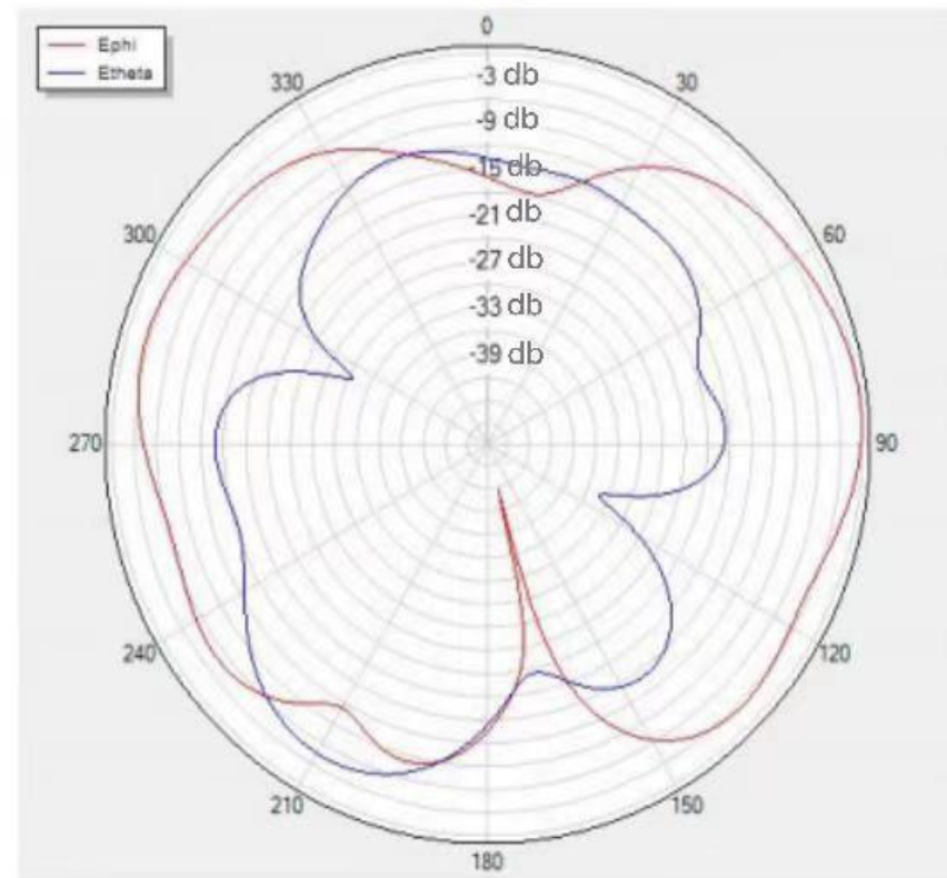
Phi=90 freq=2400MHz
