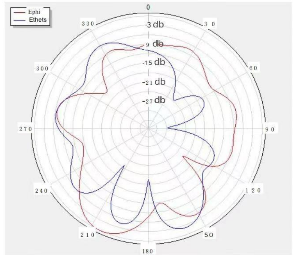
Phi=90 freq=2490MHz
