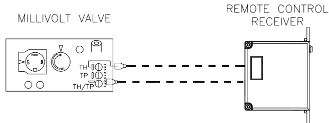
GENERIC WIRING DIAGRAM FOR RECEIVER. THE RECEIVER WIRE NEEDS TO CONNECT TO THE VALVE AT THE "TH" AND "TH/TP" JUNCTION
