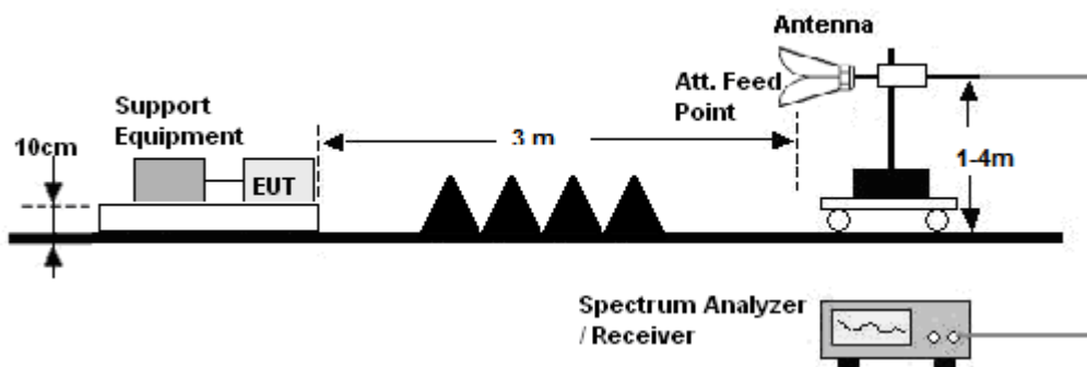
(C) Radiated Emission Test-Up Frequency Above 1GHz
