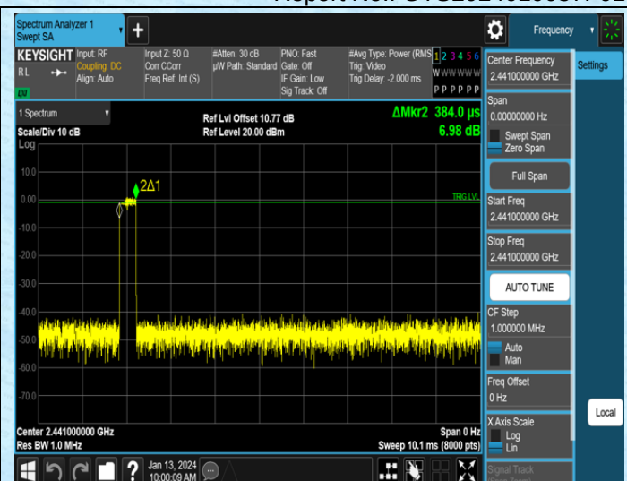
3DH1-Ant1-Hop
