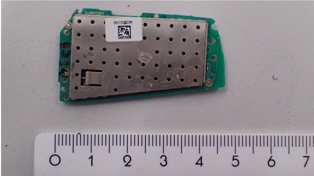
Figure 5 PCB shielded side
