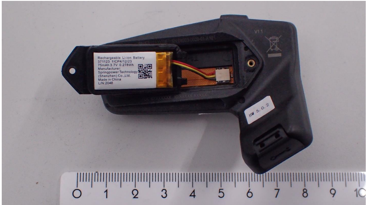
Figure 3 Battery cover open
