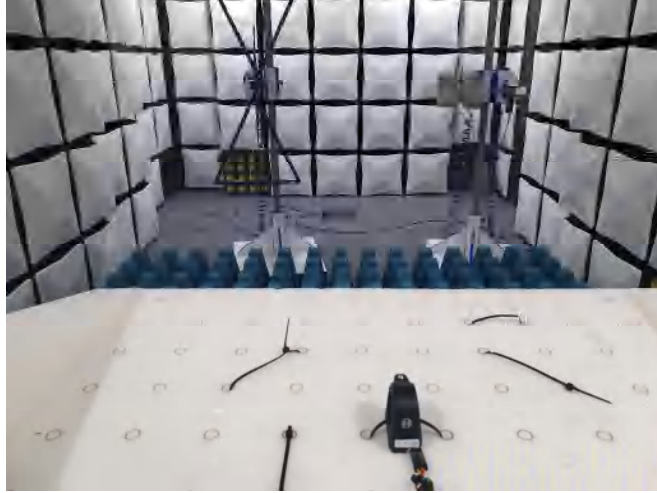
Frequency above 1GHz (FCC15C/RSS247)
