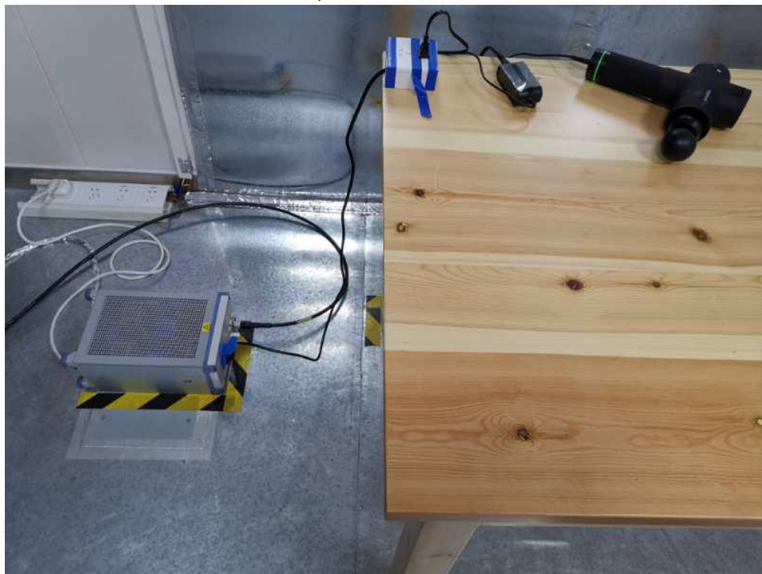
Power line conducted emission test setup
