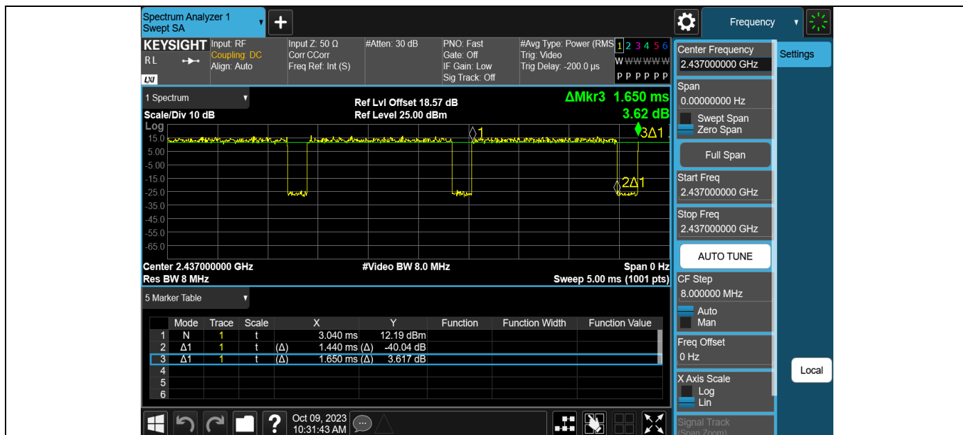
NTNV-11G-Ant2-2437
