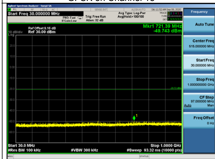
GFSK on Channel 18
