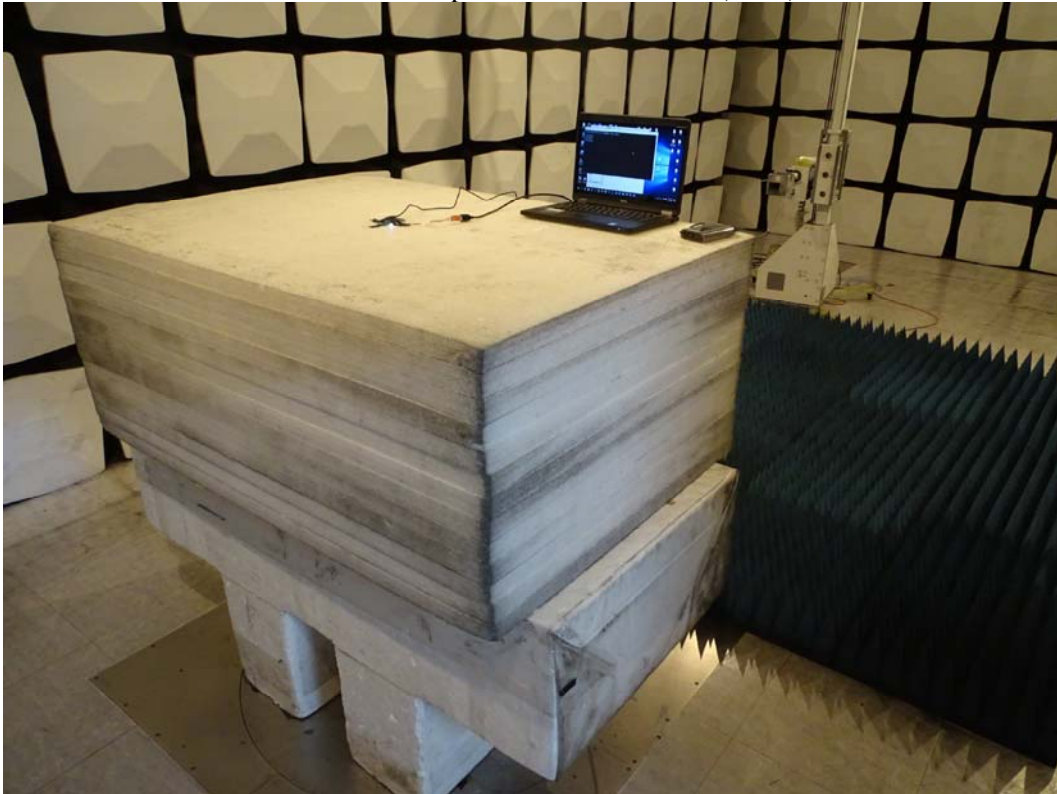
Front View of Spurious Emission Test (Horn)
