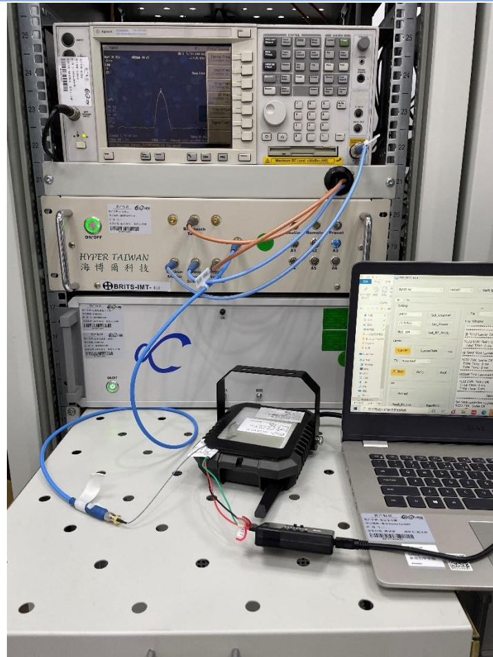
Conducted Test-BLE
