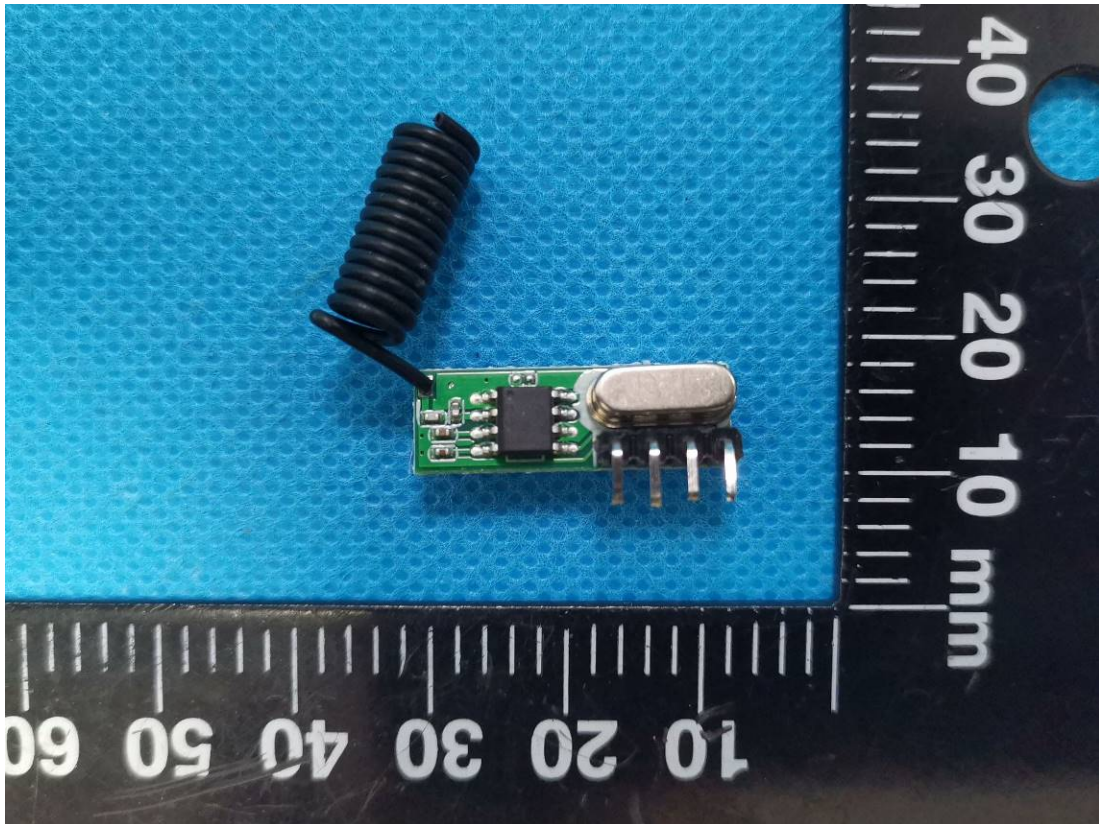
Receiver Board
