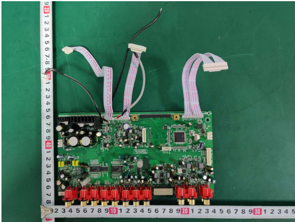
Internal photos M/N: RR2160 Mk II
