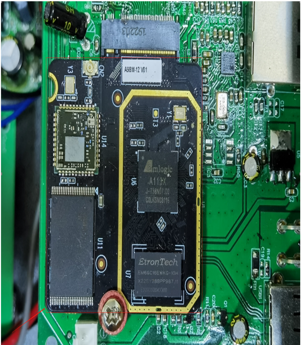
Internal photos M/N: RR2160 Mk II
