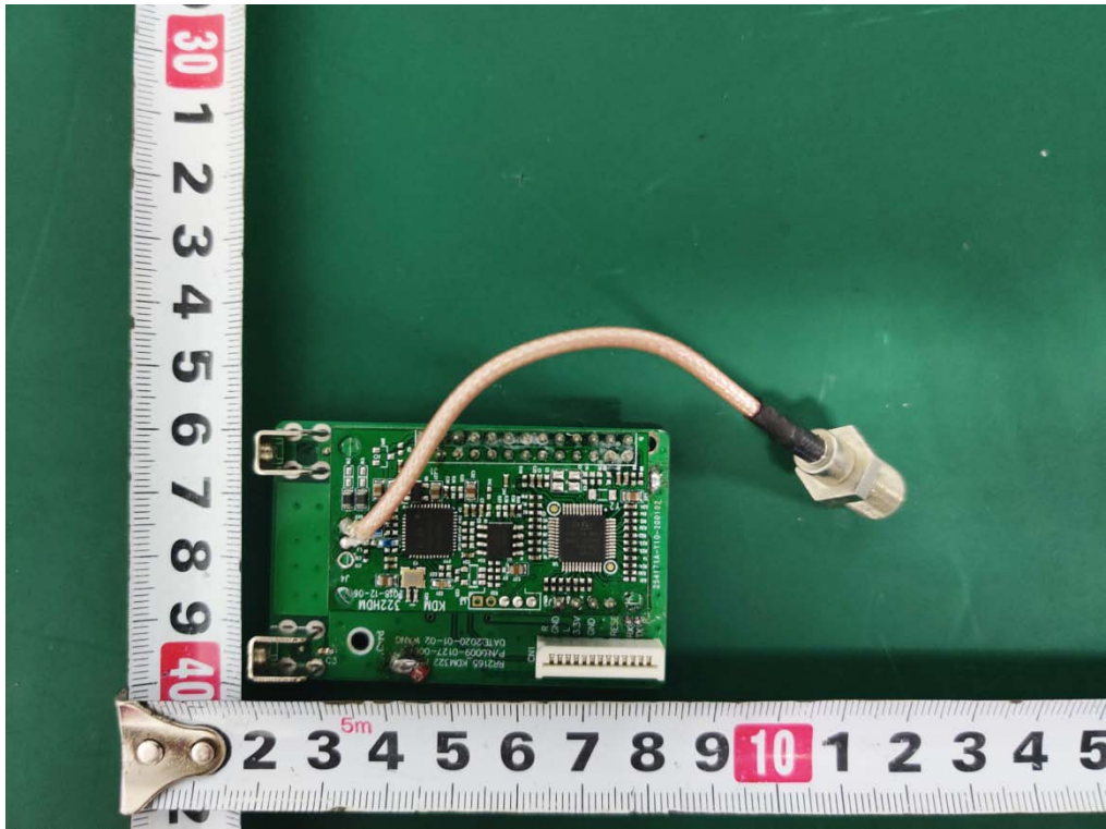
Internal photos M/N: RR2160 Mk II
