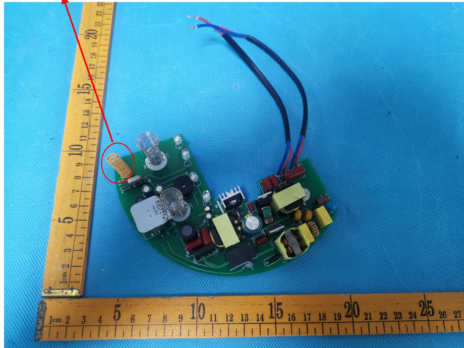
433MHz Receive ANT
