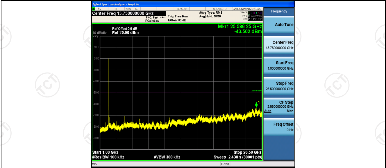
11N40SISO_Ant1_2437_0~Reference
