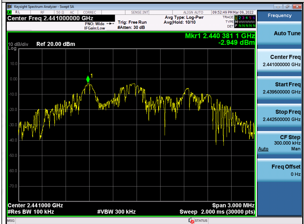
Test_Graph_LE1M_ANT1_2441_1Mbps_Reference Level
