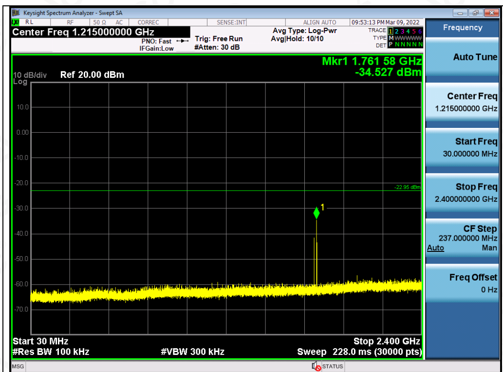
Test_Graph_LE1M_ANT1_2441_1Mbps_Lower Band Emissions
