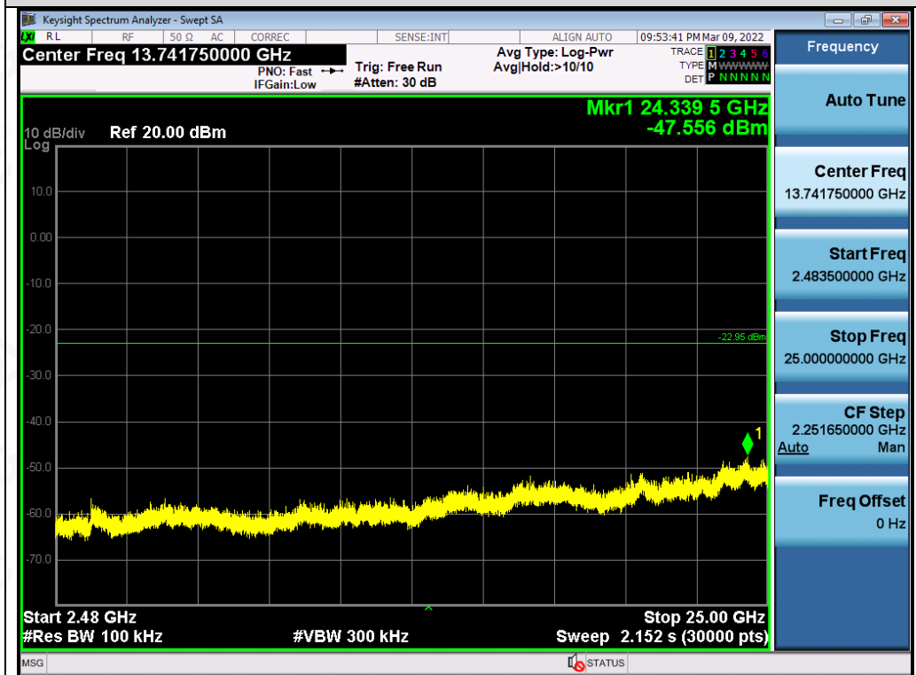
Test_Graph_LE1M_ANT1_2441_1Mbps_Higher Band Emissions
