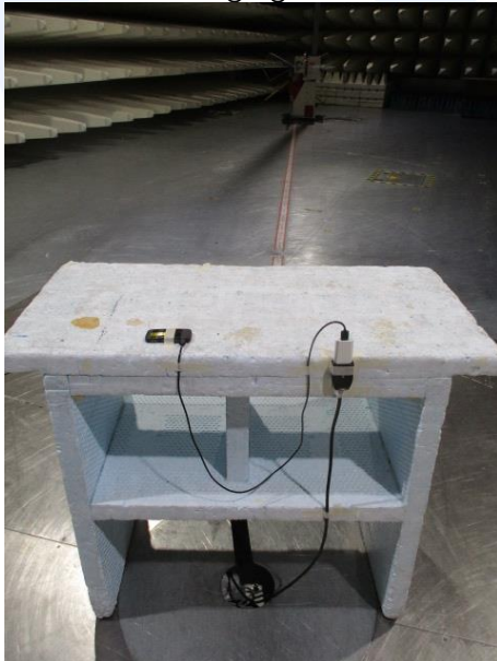
Recharging mode
