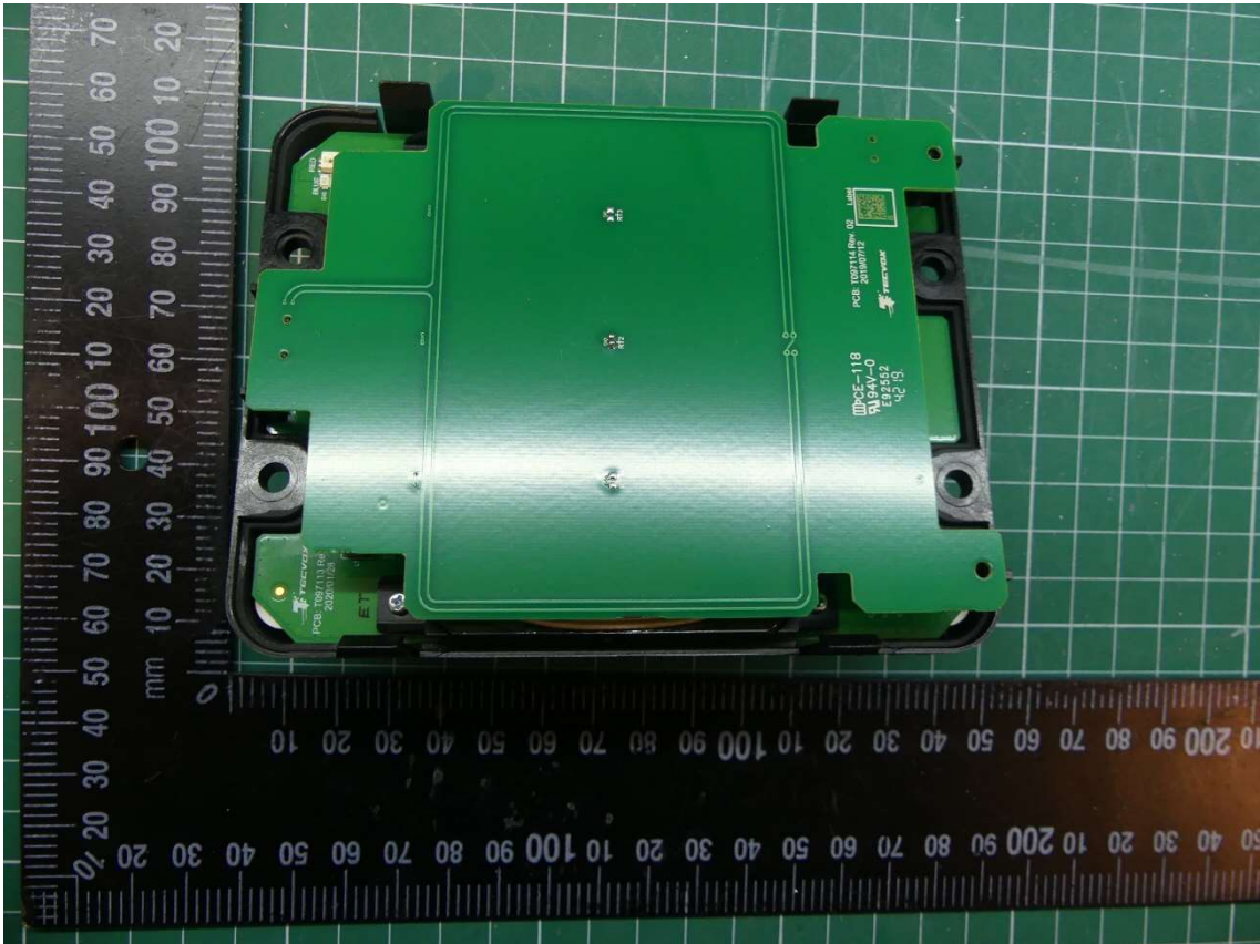
Tecvox 15W Wireless Charger – Internal pictures
