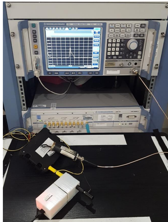
Figure B2: RFID Conducted test setup
