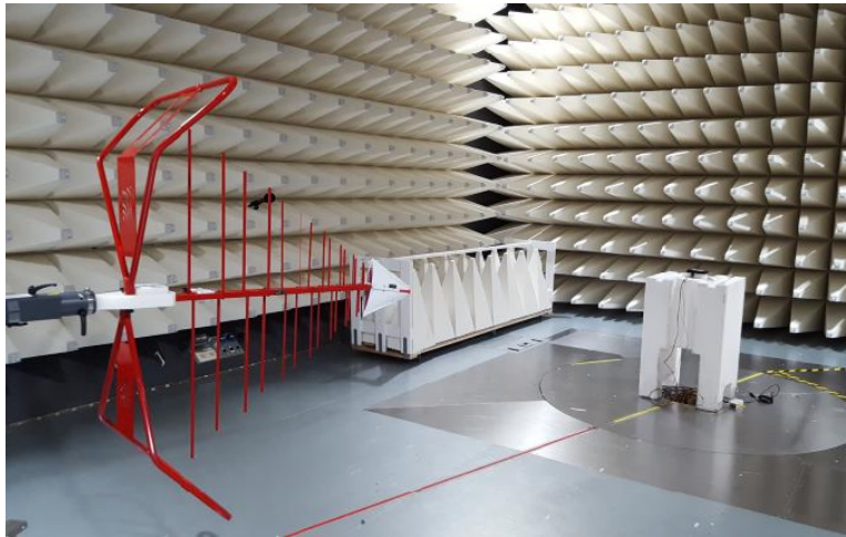
Figure B5: Radiated Emission Setup 2
