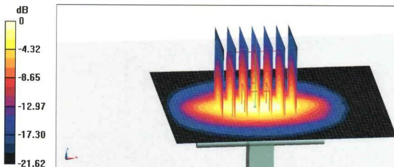
0 dB = 21.6 W/kg = 13.34 dBW/kg
