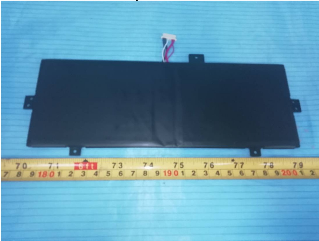
Battery: UTL-4678108-2S
