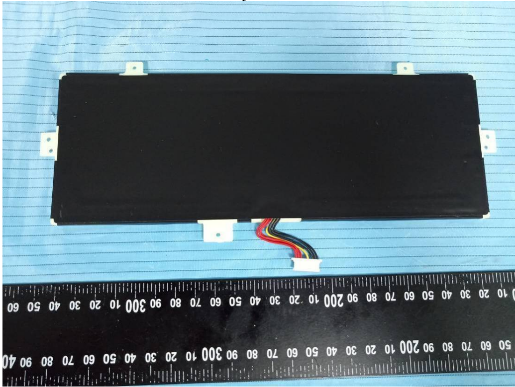
Battery: 4982229P
