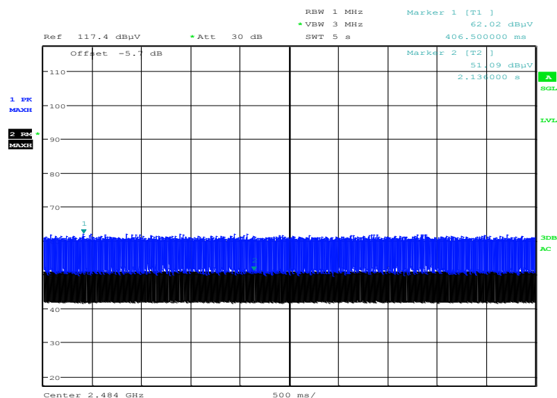
Plot 6: Upper band edge, 8 DPSK modulation, vertical & horizontal polarization, worst case
