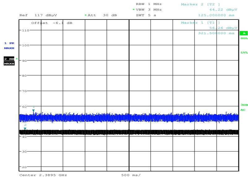
Plot 5: Lower band edge, 8 DPSK modulation, vertical & horizontal polarization, worst case
