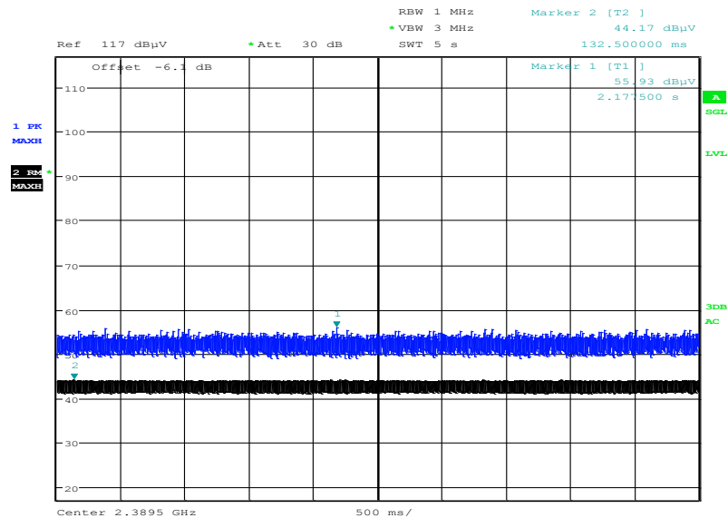
Plot 1: Lower band edge, GFSK modulation, vertical & horizontal polarization, worst case
