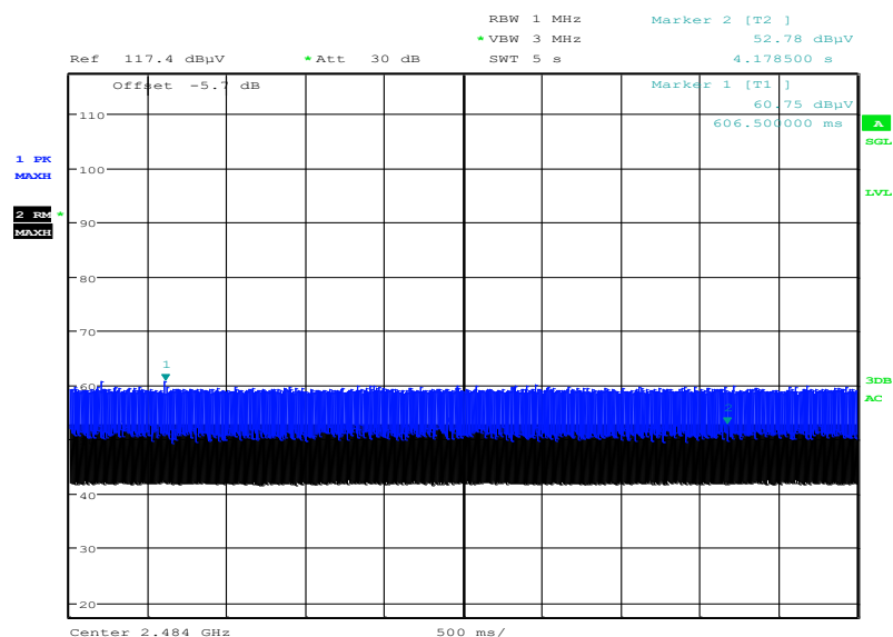
Plot 2: Upper band edge, GFSK modulation, vertical & horizontal polarization, worst case
