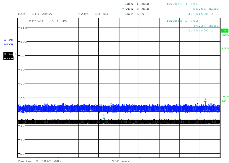
Plot 3: Lower band edge, Pi/4 DQPSK modulation, vertical & horizontal polarization, worst case
