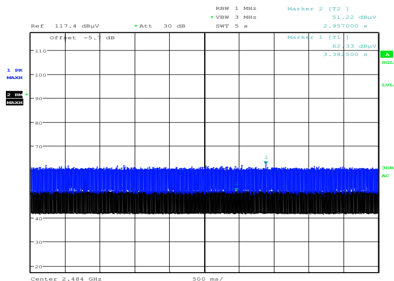
Plot 4: Upper band edge, Pi/4 DQPSK modulation, vertical & horizontal polarization, worst case
