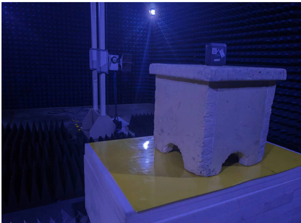
Photo of Radiated Emission Measurement (Above 960MHz)
