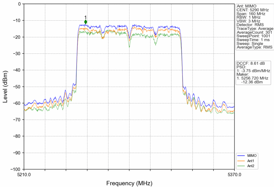
802.11ax(HEW80)_MCH_5290MHz_RU996_Left_MIMO_NTNV
