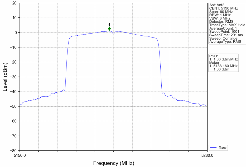
802.11ax(HEW40)_LCH_5190MHz_RU484_Left_MIMO_NTNV
