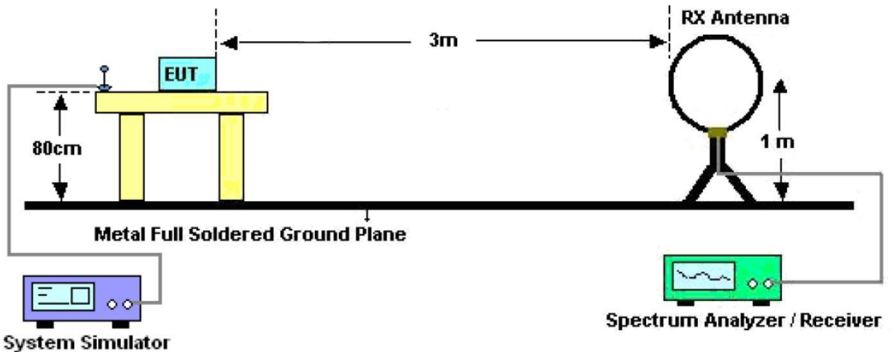
Figure 1. Below 30MHz
