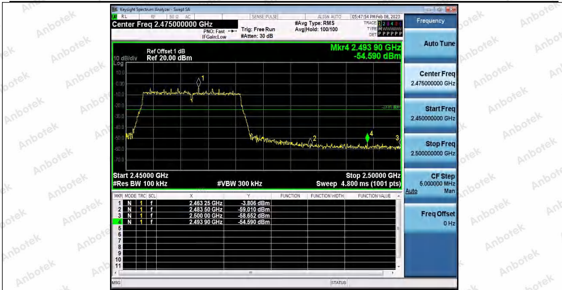
11N20_Ant2_High_2462
