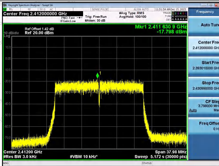
11A20SISO_Ant1_2412
