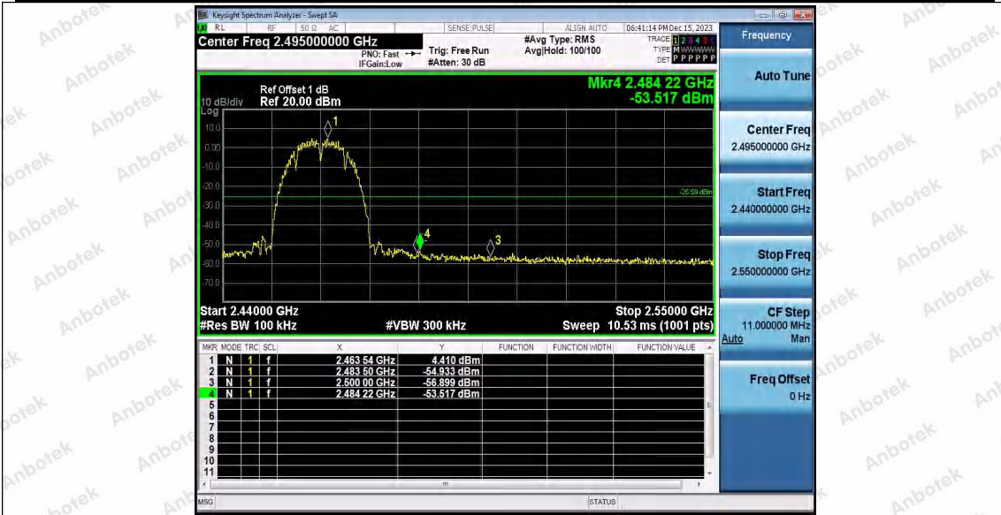
11B_Ant2_High_2462
