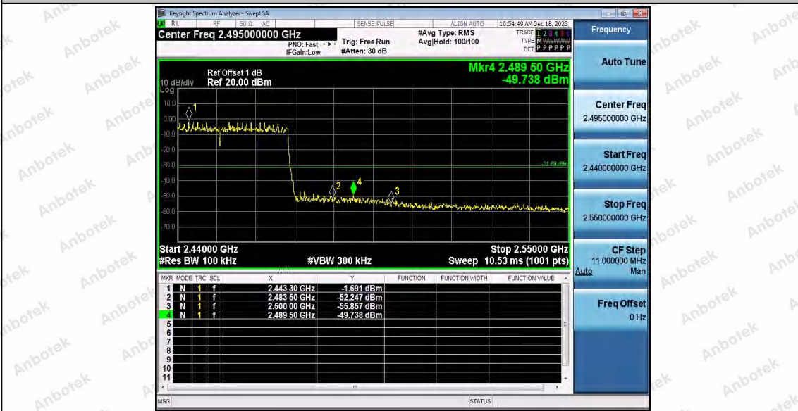
11AX40SISO_Ant2_High_2452
