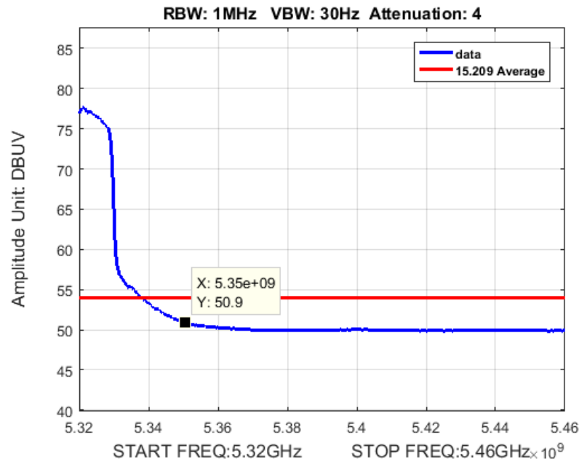
Figure 21: Band Edge BW 20M Ch 5320M 80211n Average
