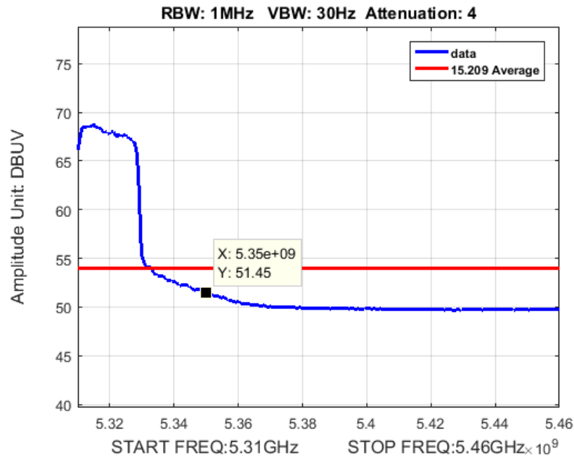
Figure 23: Band Edge BW 40M Ch 5310M 80211n Average
