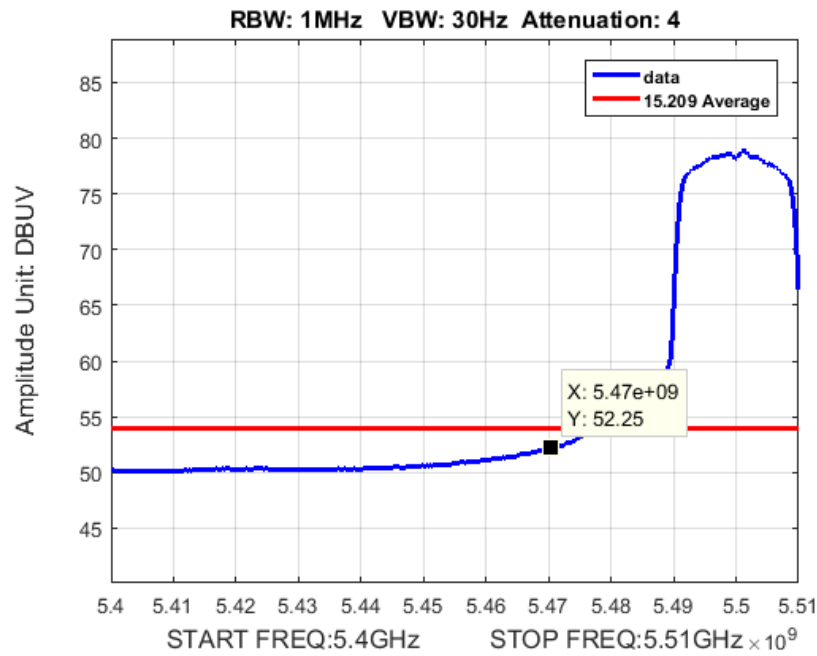
Figure 29: Band Edge BW 20M Ch 5500M 80211n Average
