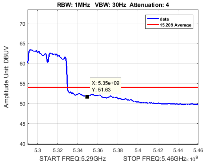
Figure 25: Band Edge BW 80M Ch 5290M 80211ac Average
