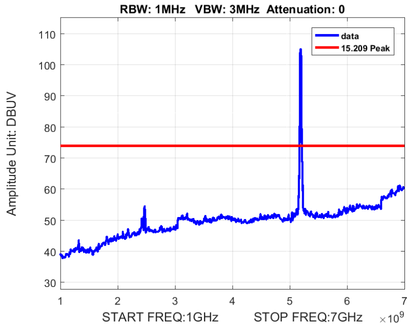
Figure 6: Radiated Spurious Emissions 1-7GHz BW 40M Ch 5190M 802.11n Peak
