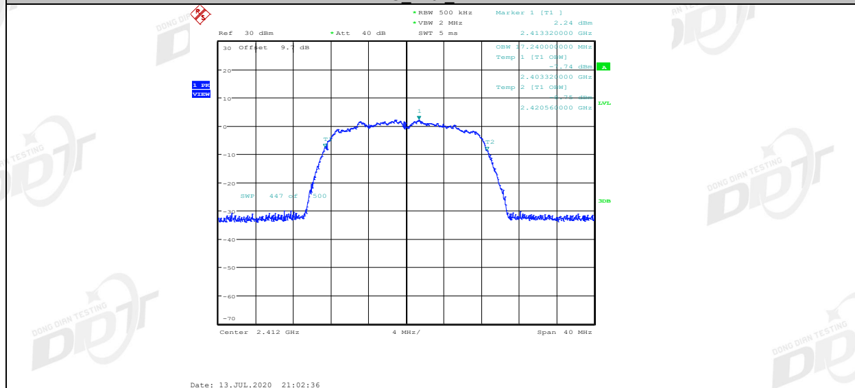
11G Ant2 2412
