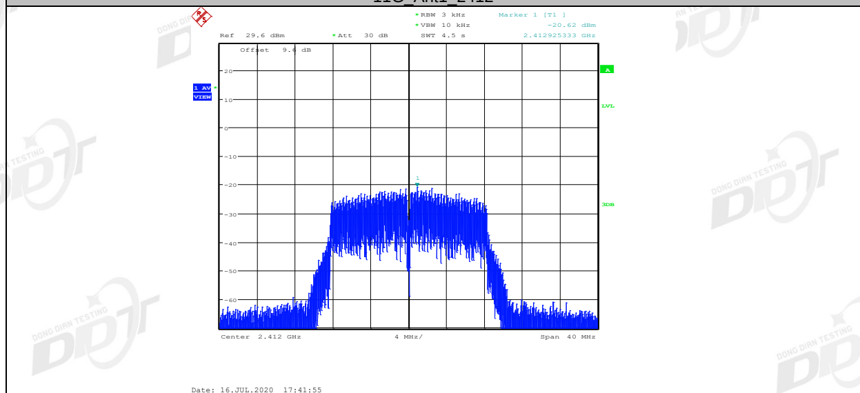
11G Ant2 2412
