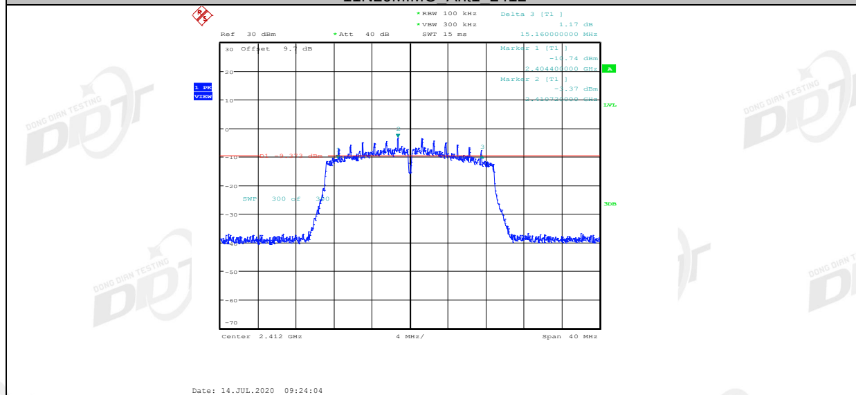
11N20MIMO Ant2 2412
