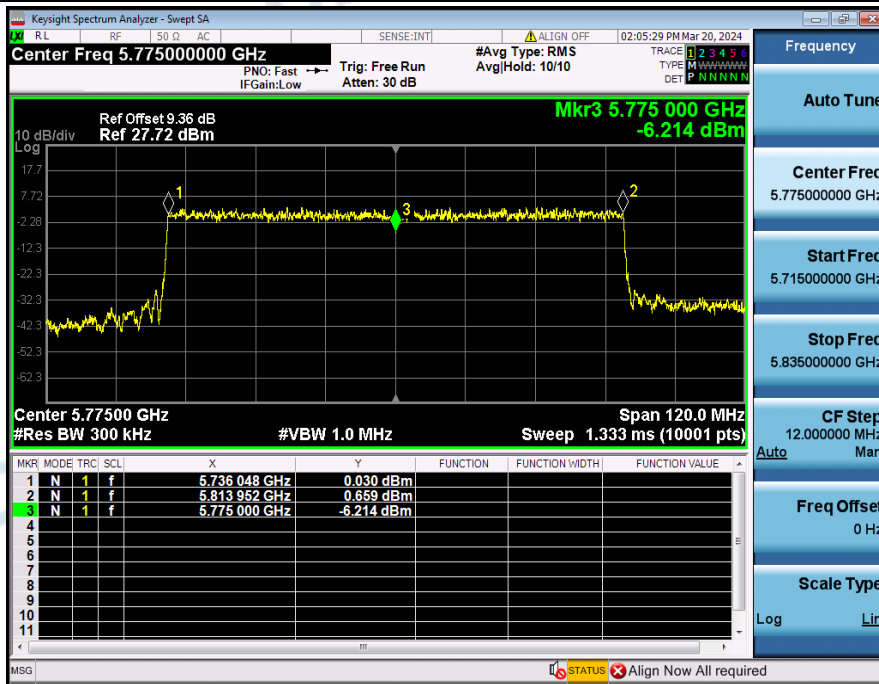
Frequency_Stability_NVNT_ANT3_802_11ax(HE80)_5775
