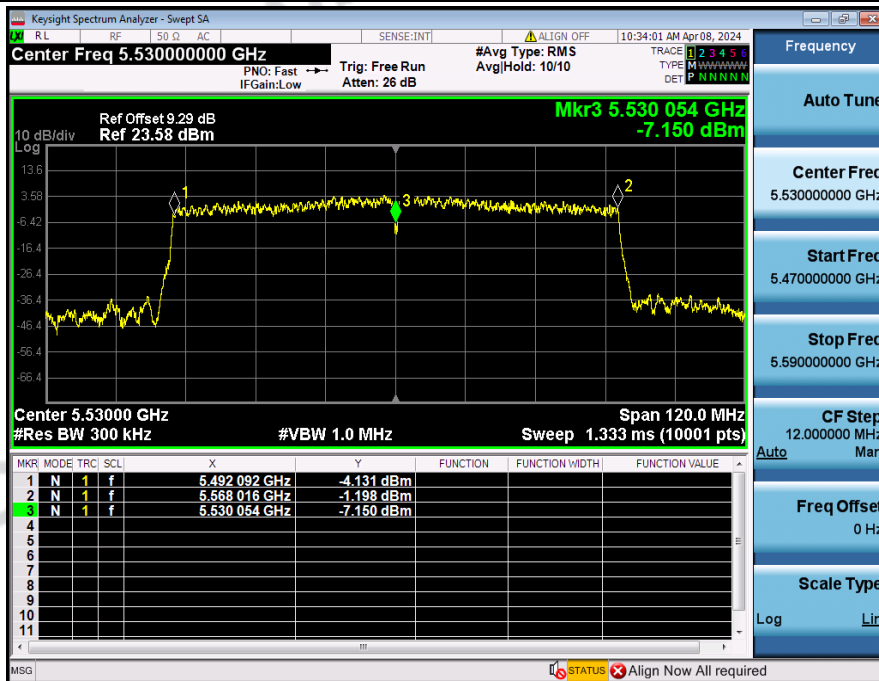
Frequency_Stability_NVNT_ANT3_802_11ac(VHT80)_5530
