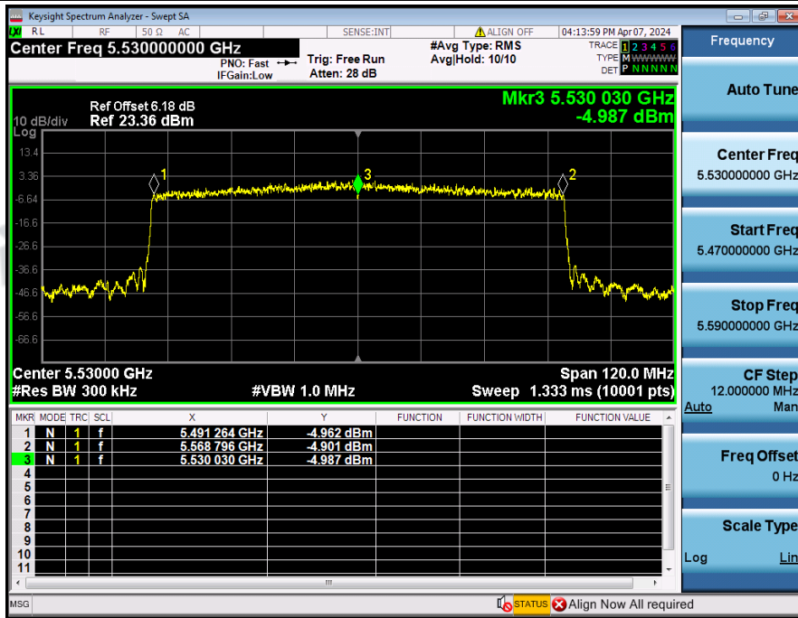
Frequency_Stability_NVNT_ANT2_802_11ax(HE80)_5530
