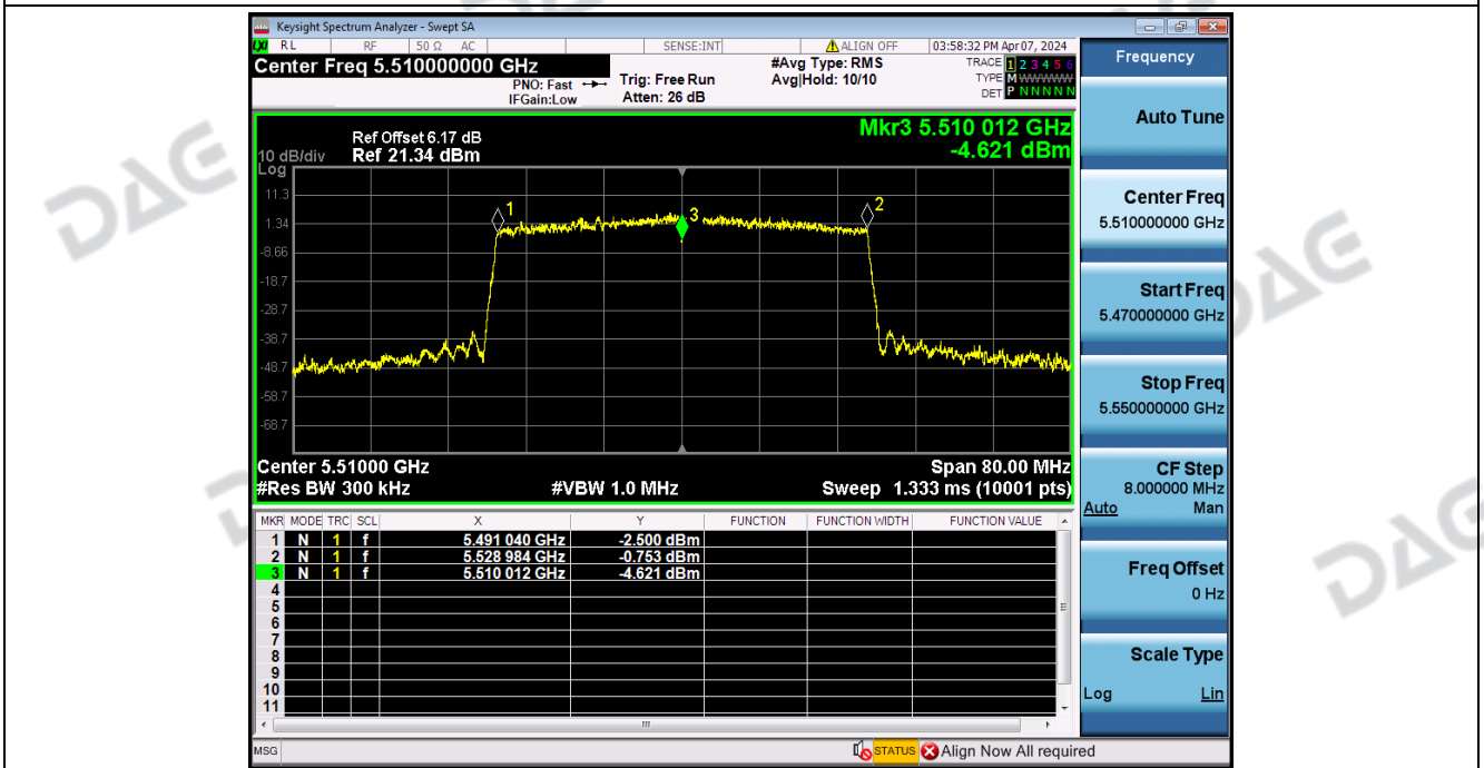
Frequency_Stability_NVNT_ANT2_802_11ax(HE40)_5510
