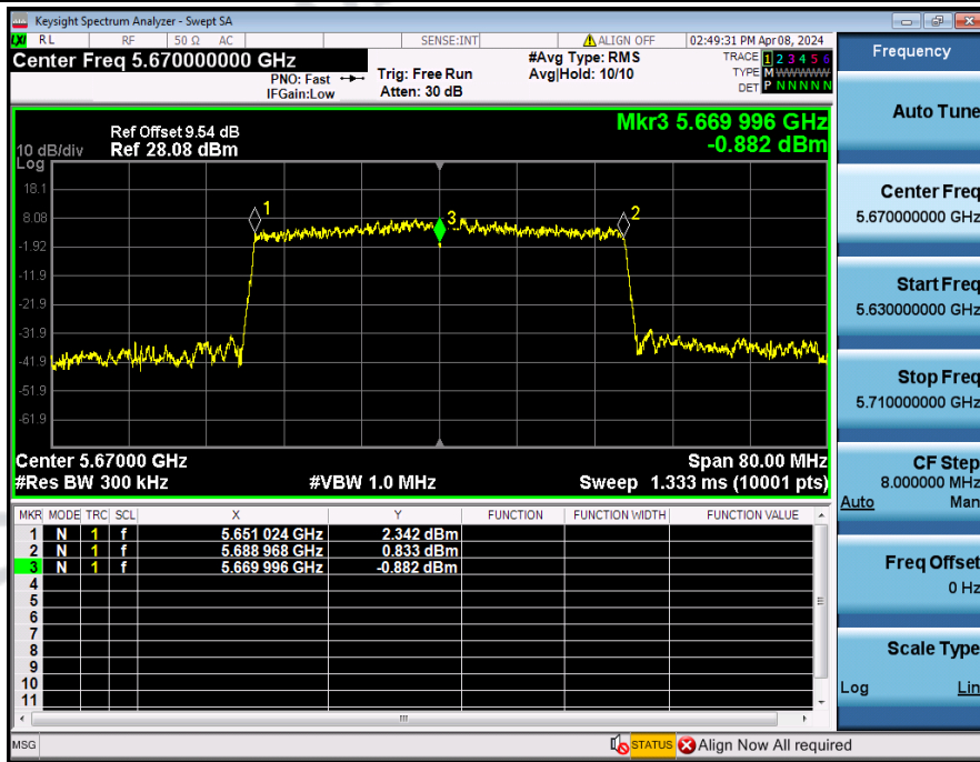
Frequency_Stability_NVNT_ANT3_802_11ax(HE40)_5670
