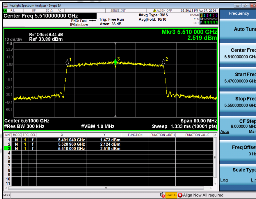
Frequency_Stability_NVNT_ANT3_802_11ax(HE40)_5510
