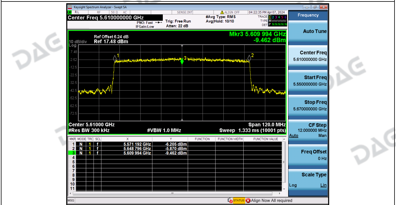
Frequency_Stability_NVNT_ANT2_802_11ax(HE80)_5610
