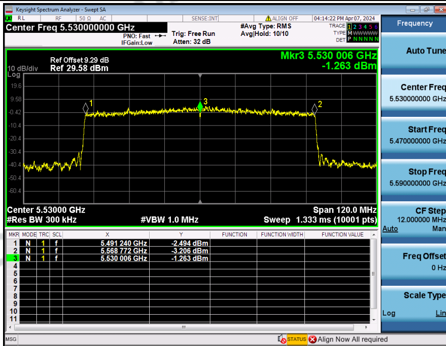
Frequency_Stability_NVNT_ANT3_802_11ax(HE80)_5530
