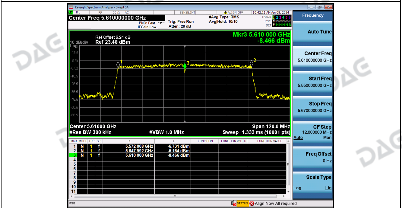
Frequency_Stability_NVNT_ANT2_802_11ac(VHT80)_5610
