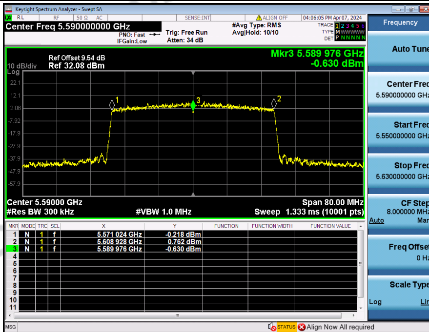
Frequency_Stability_NVNT_ANT3_802_11ax(HE40)_5590
