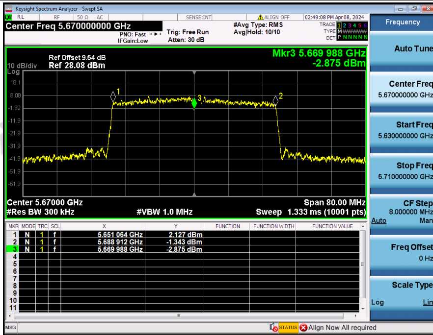
Frequency_Stability_NVNT_ANT3_802_11ax(HE40)_5670
