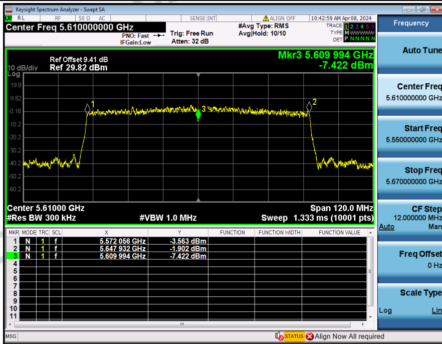
Frequency_Stability_NVNT_ANT3_802_11ac(VHT80)_5610
