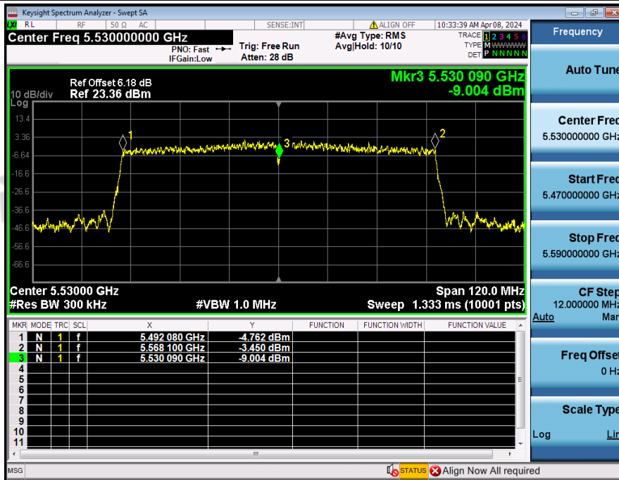
Frequency_Stability_NVNT_ANT2_802_11ac(VHT80)_5530
