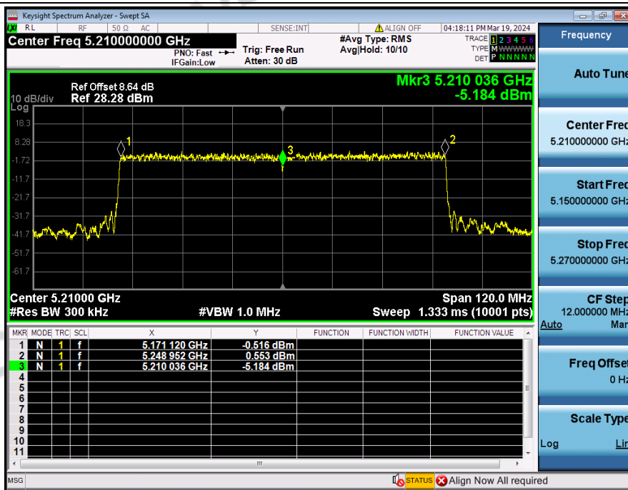
Frequency_Stability_NVNT_ANT3_802_11ax(HE80)_5210
