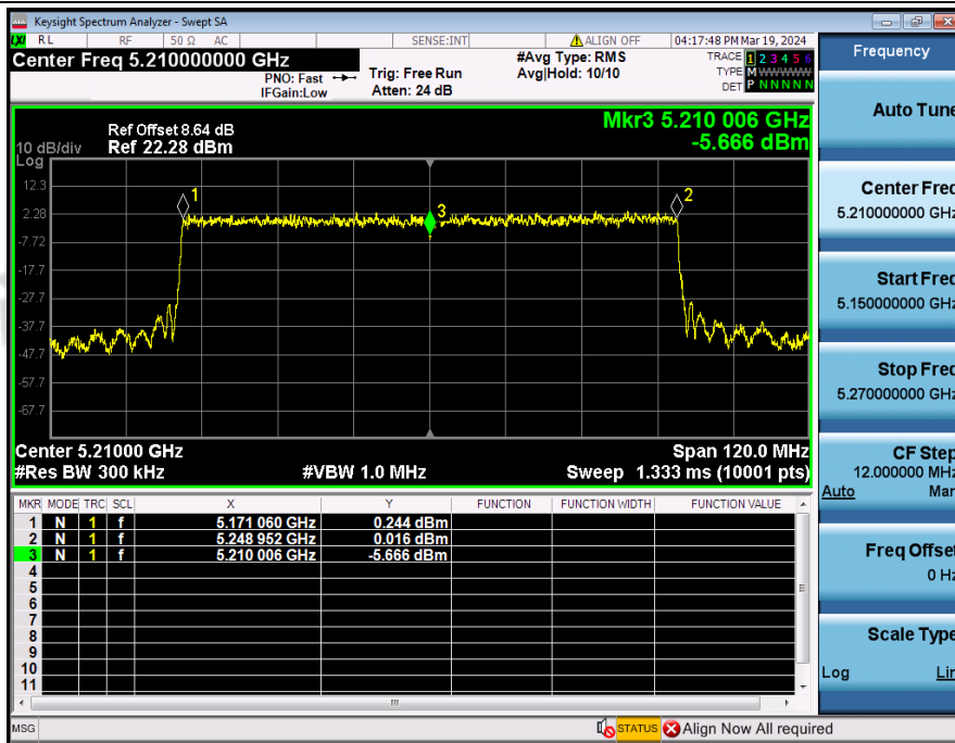
Frequency_Stability_NVNT_ANT3_802_11ax(HE80)_5210
