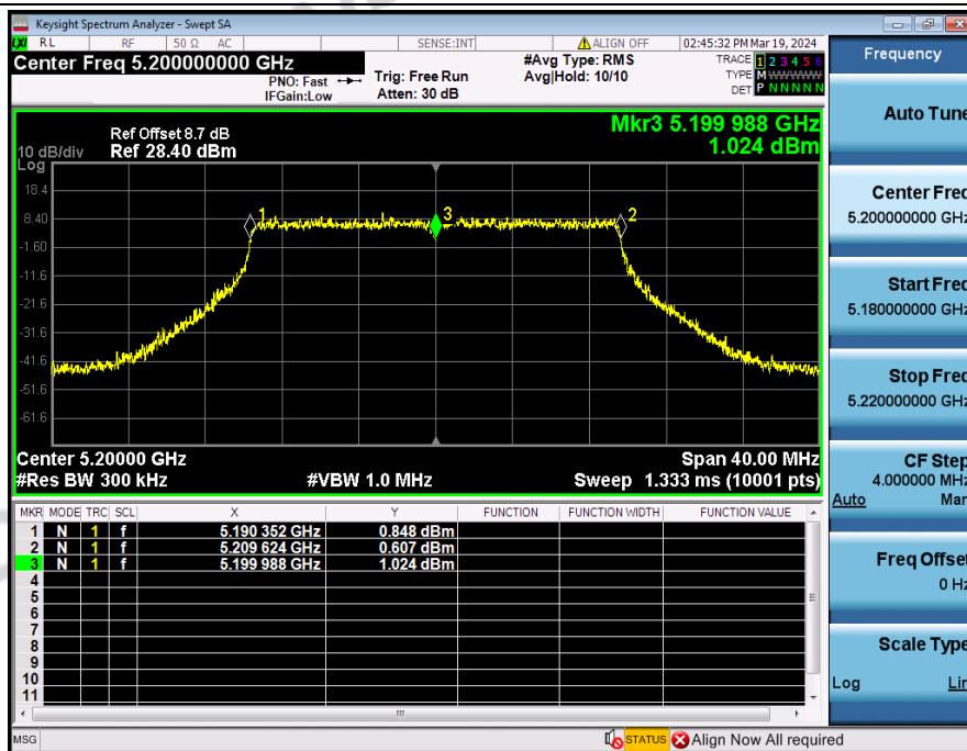
Frequency_Stability_NVNT_ANT3_802_11ax(HE20)_5200
