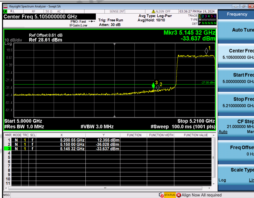
Bandedge_NVNT_ANT3_802_11ax(HE40)_5190
