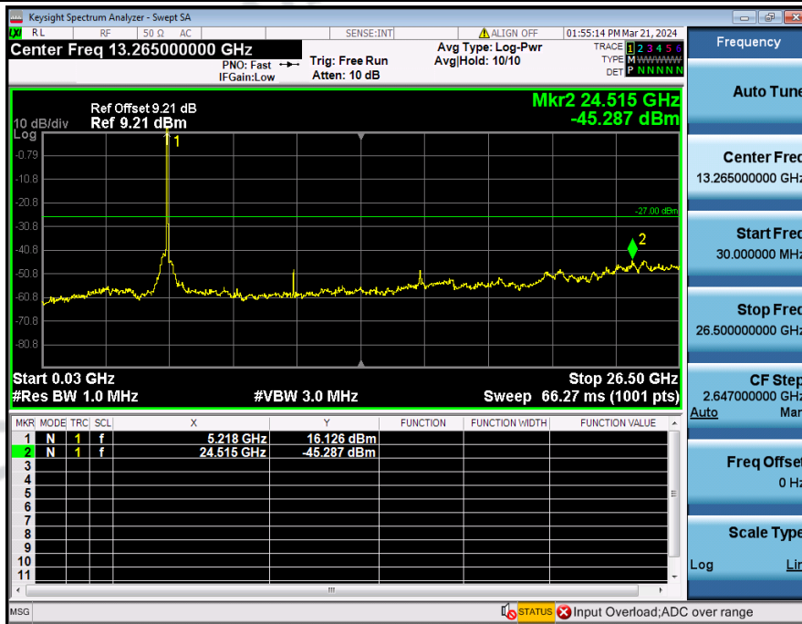
Spurious_Emission_NVNT_3TXx3RX_802_11ac(VHT20)_5240_20M
