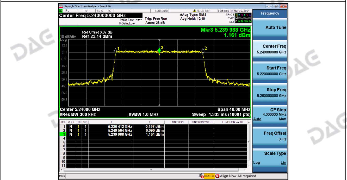
Frequency_Stability_NVNT_ANT2_802_11ax(HE20)_5240
