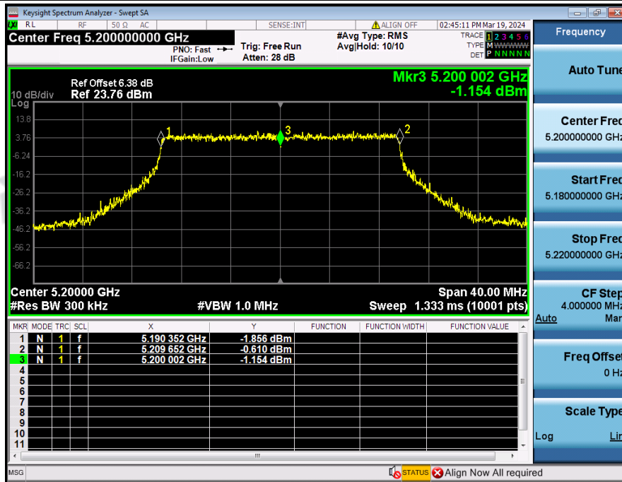
Frequency_Stability_NVNT_ANT2_802_11ax(HE20)_5200
