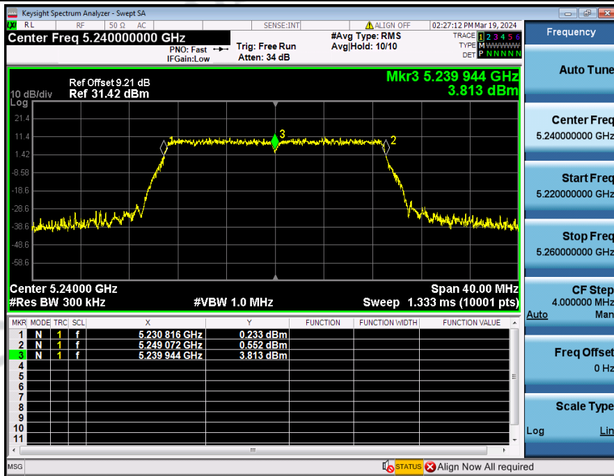
Frequency_Stability_NVNT_ANT3_802_11ac(VHT20)_5240
