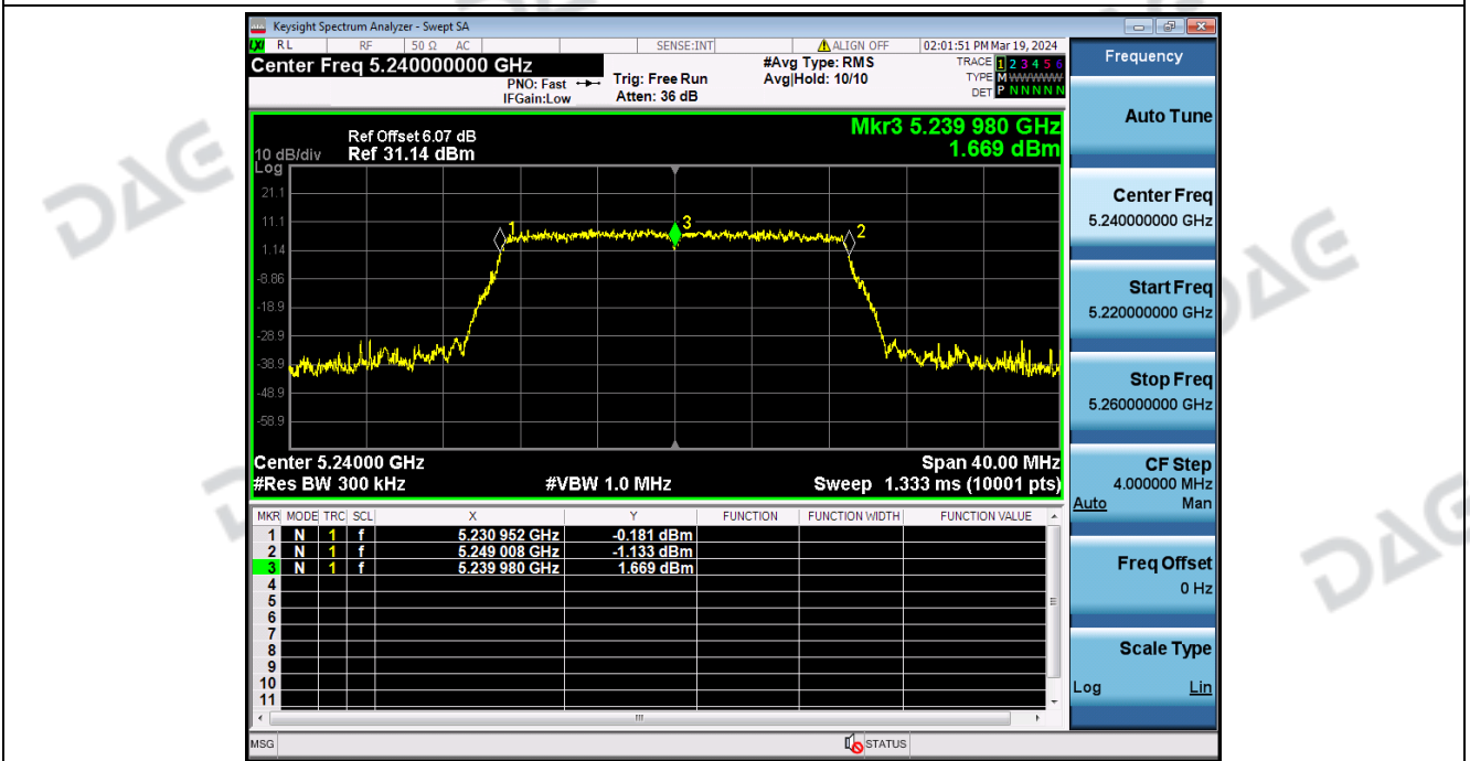
Frequency_Stability_NVNT_ANT2_802_11n(HT20)_5240
