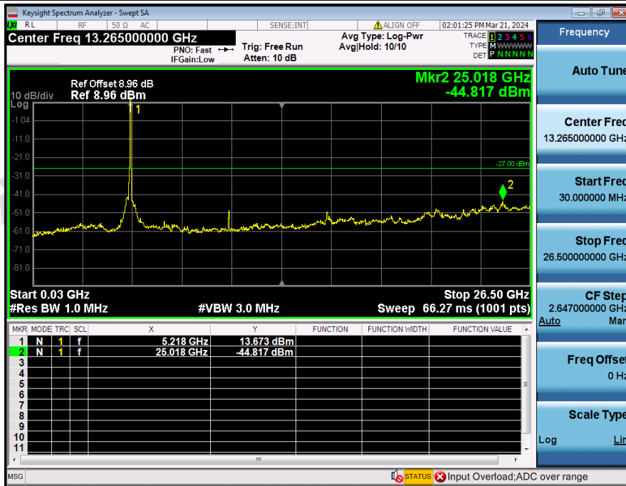
Spurious_Emission_NVNT_3TXx3RX_802_11n(HT40)_5230_40M
