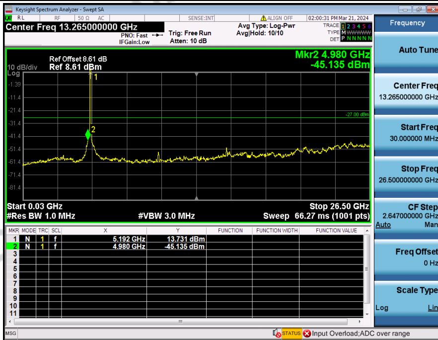
Spurious_Emission_NVNT_3TXx3RX_802_11n(HT40)_5190_40M
