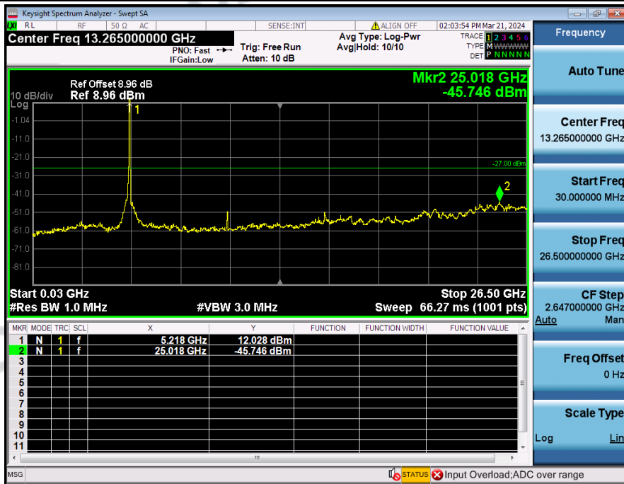
Spurious_Emission_NVNT_3TXx3RX_802_11ac(VHT40)_5230_40M
