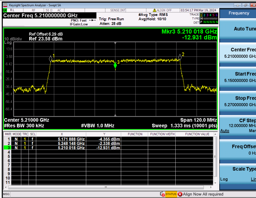
Frequency_Stability_NVNT_ANT2_802_11ac(VHT80)_5210
