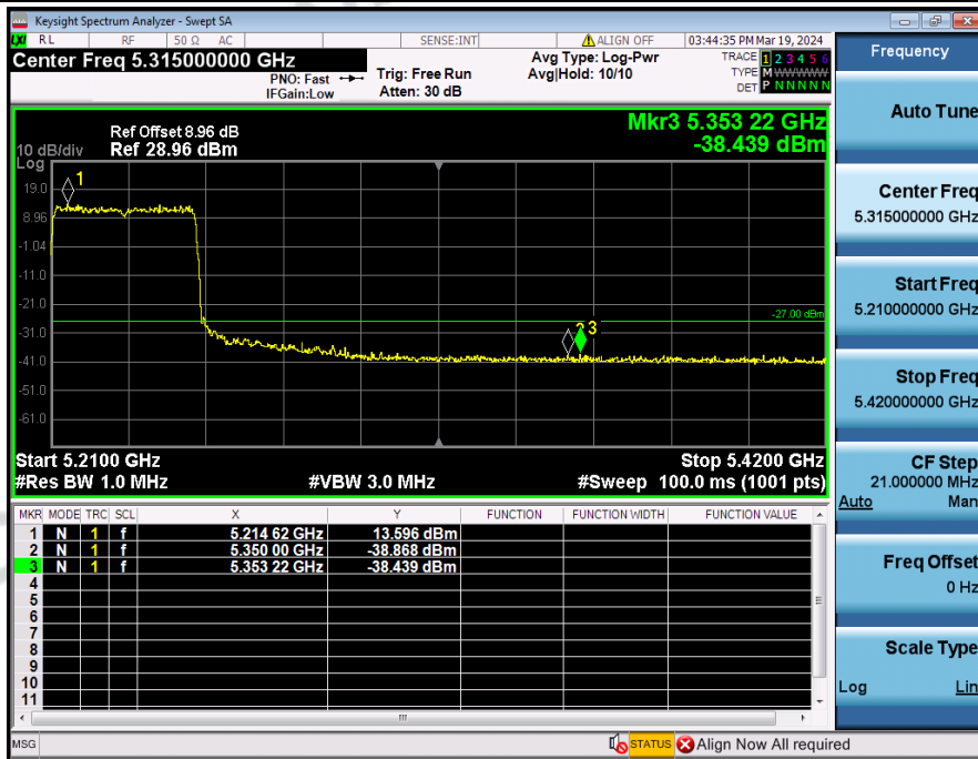
Bandedge_NVNT_ANT3_802_11ax(HE40)_5230
