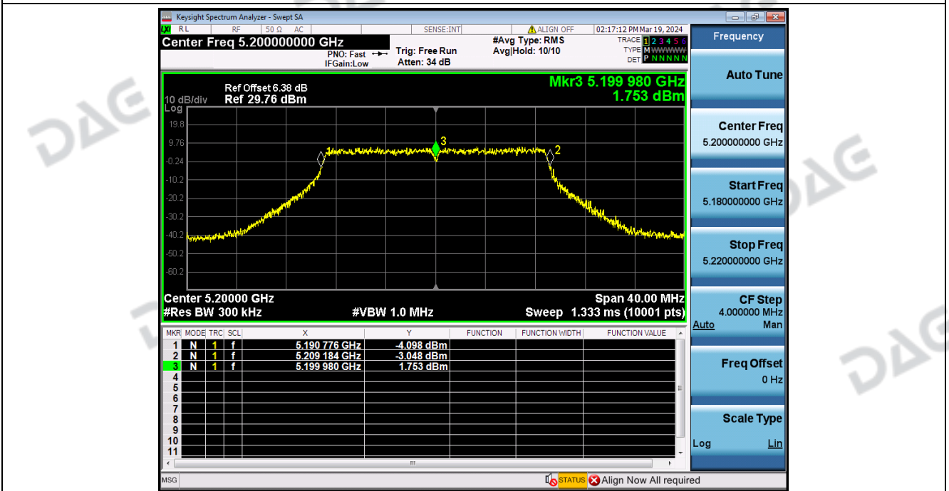
Frequency_Stability_NVNT_ANT2_802_11ac(VHT20)_5200
