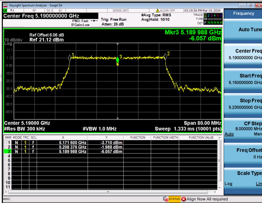
Frequency_Stability_NVNT_ANT2_802_11ac(VHT40)_5190
