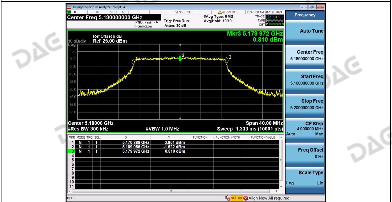
Frequency_Stability_NVNT_ANT2_802_11n(HT20)_5180
