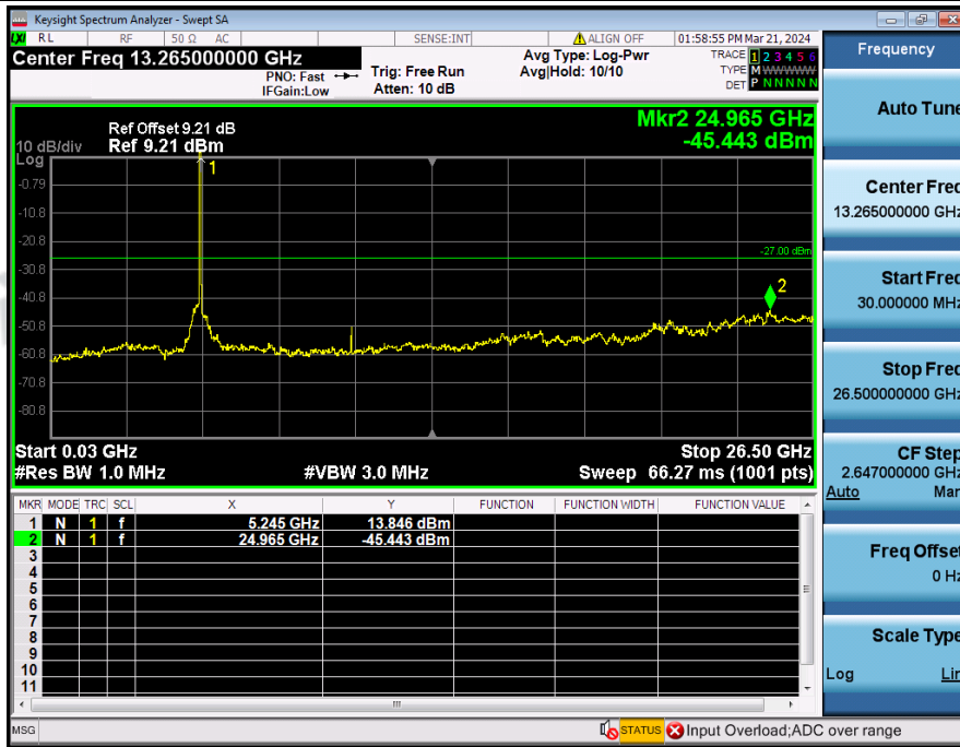
Spurious_Emission_NVNT_3TXx3RX_802_11ax(HE20)_5240_20M
