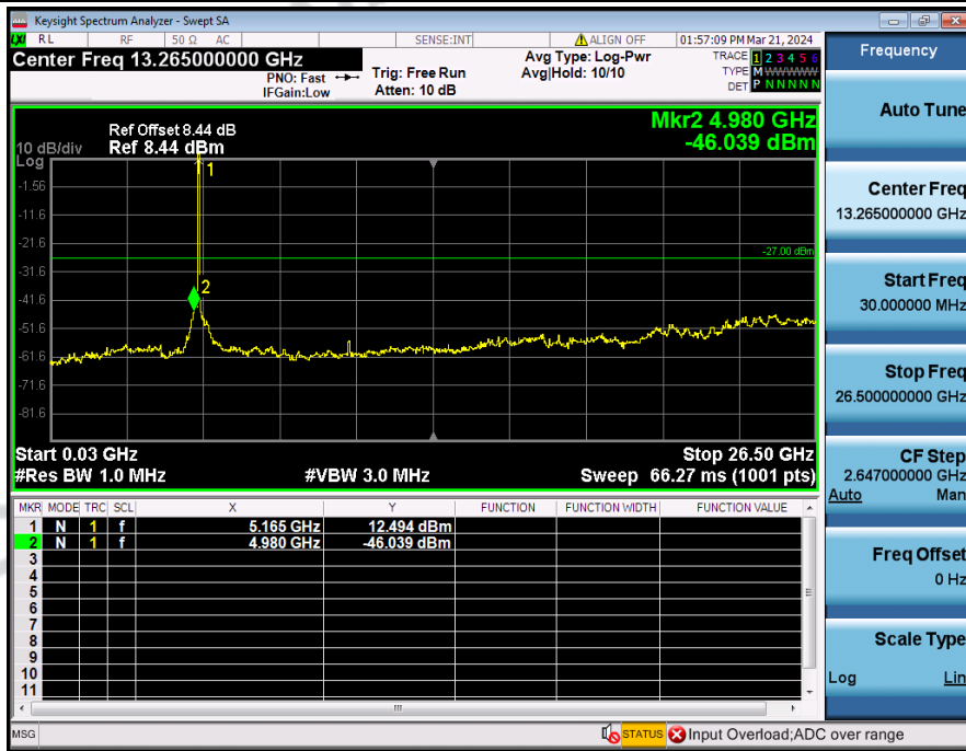
Spurious_Emission_NVNT_3TXx3RX_802_11ax(HE20)_5180_20M
