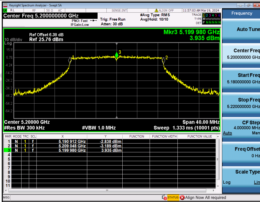
Frequency_Stability_NVNT_ANT2_802_11n(HT20)_5200
