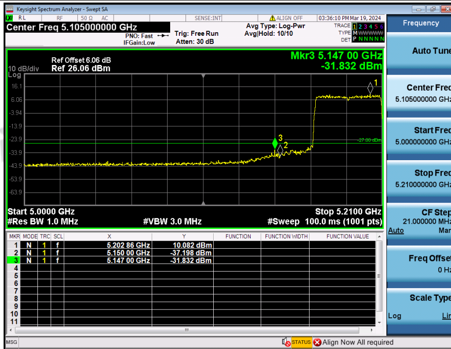
Bandedge_NVNT_ANT2_802_11ax(HE40)_5190
