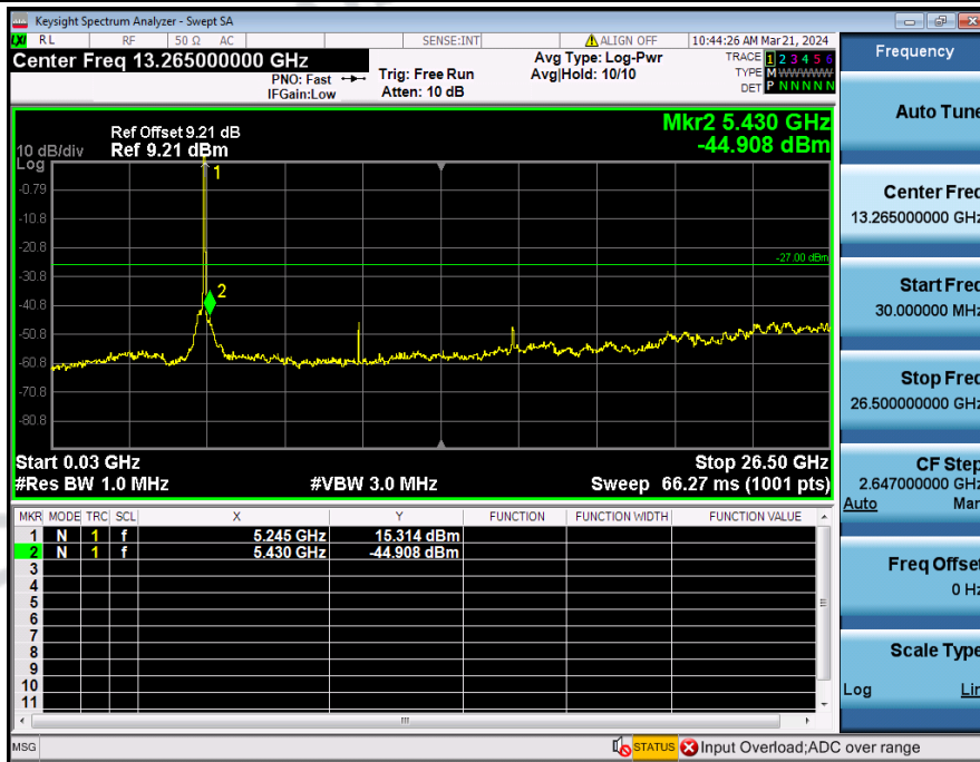
Spurious_Emission_NVNT_3TXx3RX_802_11a_5240_20M
