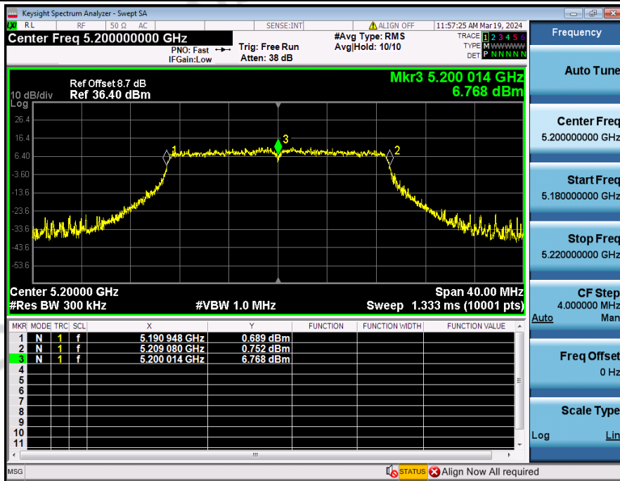
Frequency_Stability_NVNT_ANT3_802_11n(HT20)_5200
