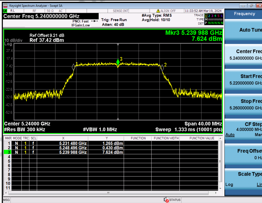
Frequency_Stability_NVNT_ANT3_802_11a_5240
