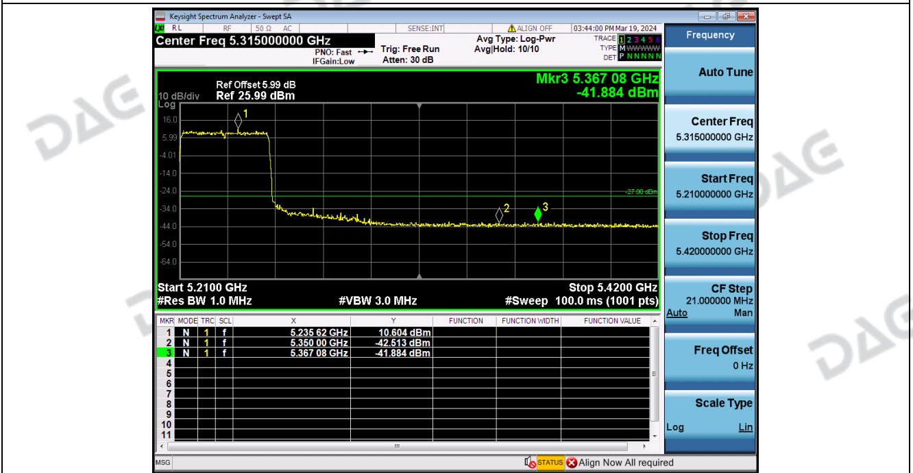
Bandedge_NVNT_ANT2_802_11ax(HE40)_5230
