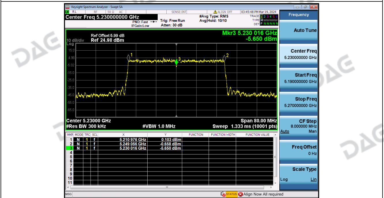
Frequency_Stability_NVNT_ANT2_802_11ax(HE40)_5230
