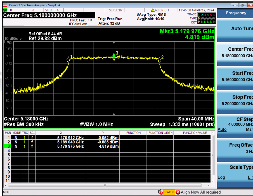
Frequency_Stability_NVNT_ANT3_802_11n(HT20)_5180
