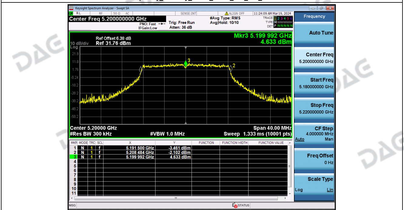
Frequency_Stability_NVNT_ANT2_802_11a_5200
