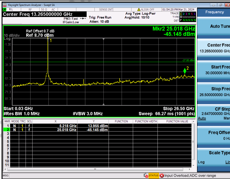
Spurious_Emission_NVNT_3TXx3RX_802_11ac(VHT20)_5200_20M
