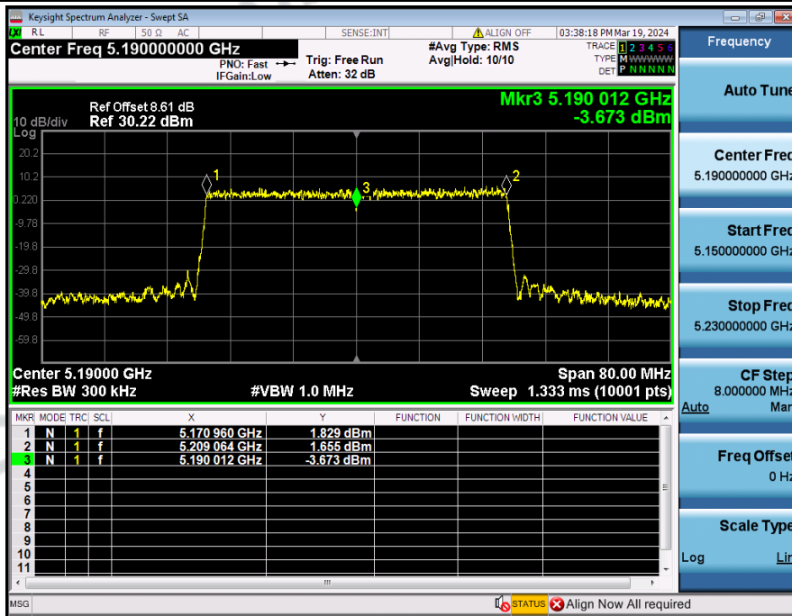
Frequency_Stability_NVNT_ANT3_802_11ax(HE40)_5190
