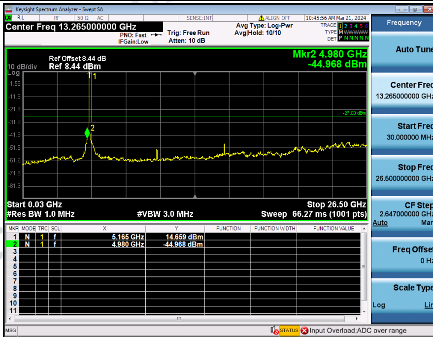
Spurious_Emission_NVNT_3TXx3RX_802_11n(HT20)_5180_20M
