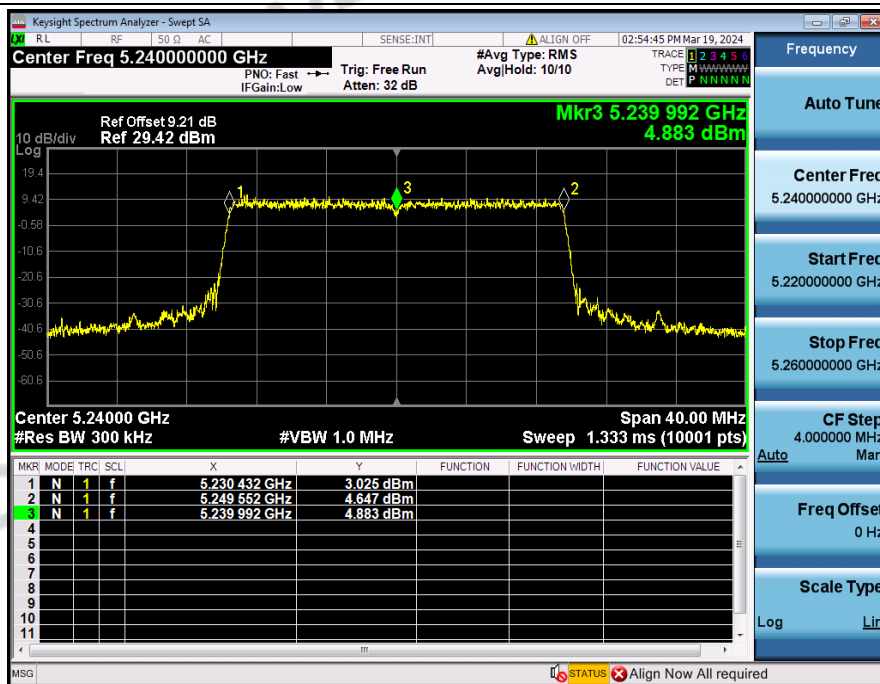
Frequency_Stability_NVNT_ANT3_802_11ax(HE20)_5240
