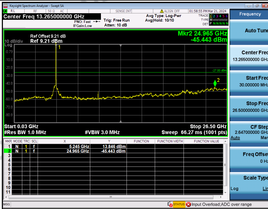
Spurious_Emission_NVNT_3TXx3RX_802_11ax(HE20)_5240_20M
