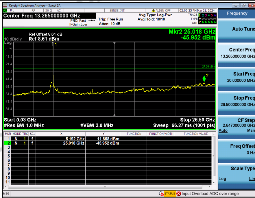
Spurious_Emission_NVNT_3TXx3RX_802_11ax(HE40)_5190_40M
