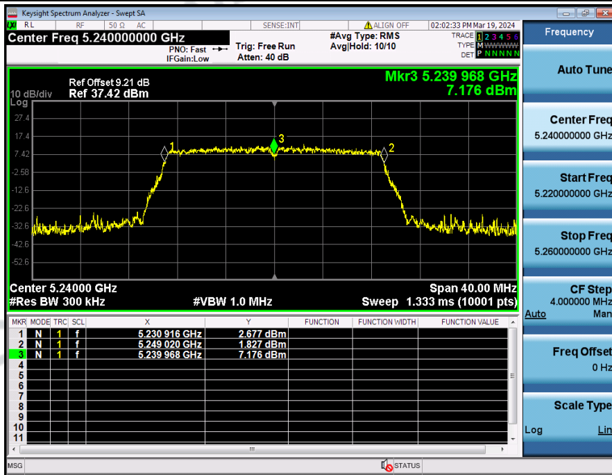
Frequency_Stability_NVNT_ANT3_802_11n(HT20)_5240
