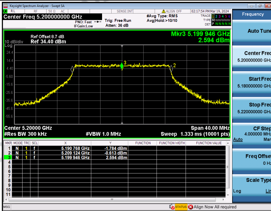
Frequency_Stability_NVNT_ANT3_802_11ac(VHT20)_5200
