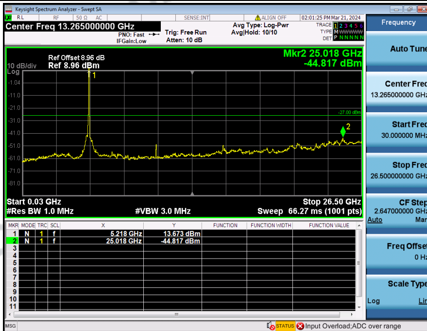
Spurious_Emission_NVNT_3TXx3RX_802_11n(HT40)_5230_40M
