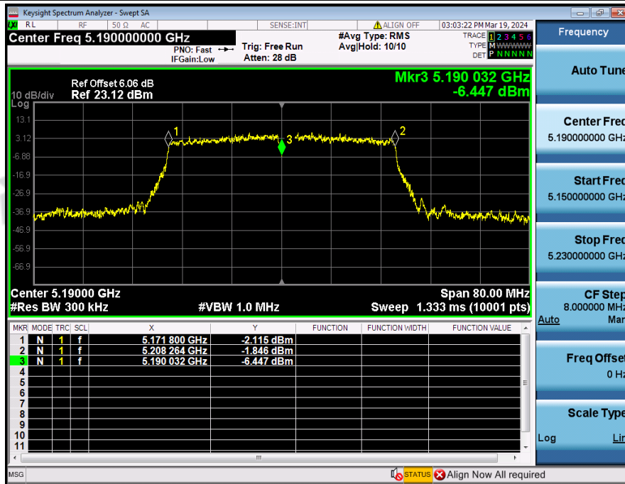
Frequency_Stability_NVNT_ANT2_802_11n(HT40)_5190
