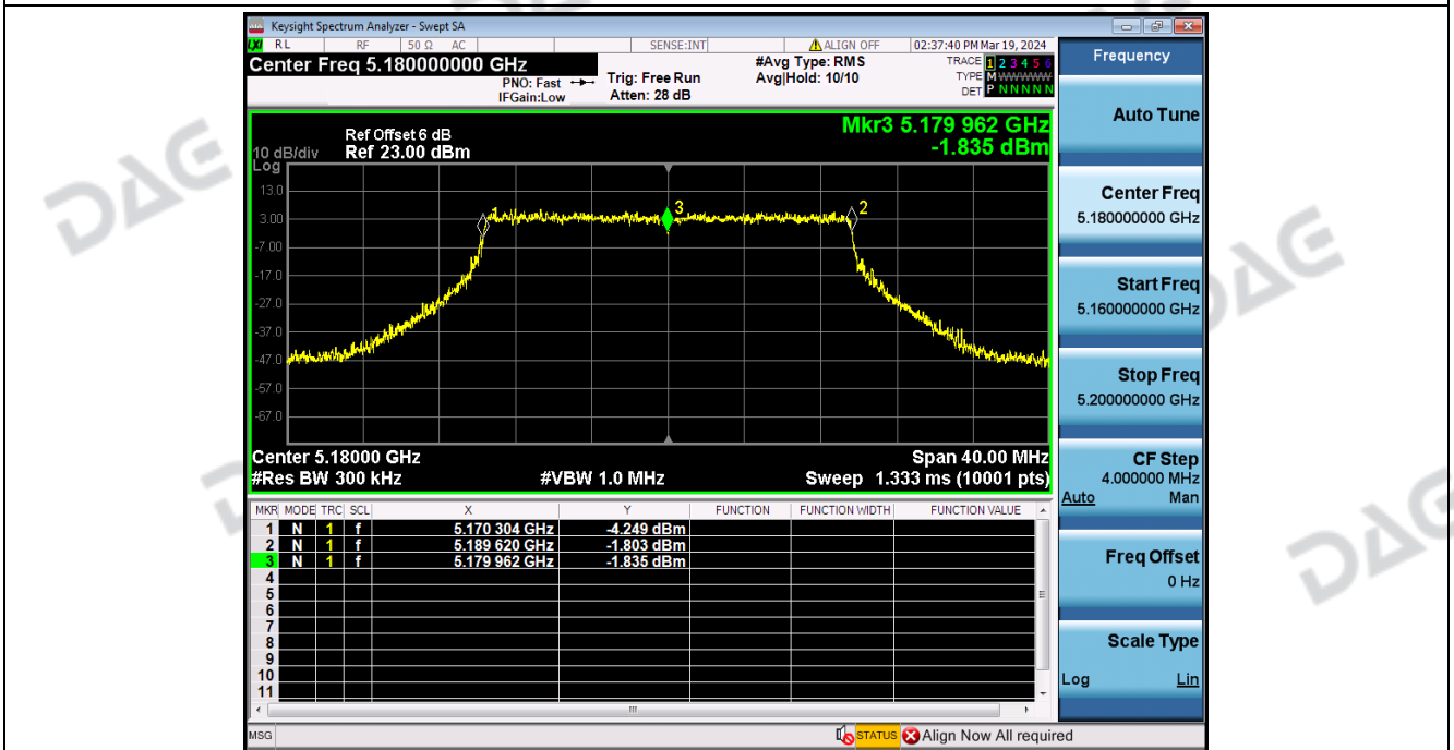
Frequency_Stability_NVNT_ANT2_802_11ax(HE20)_5180
