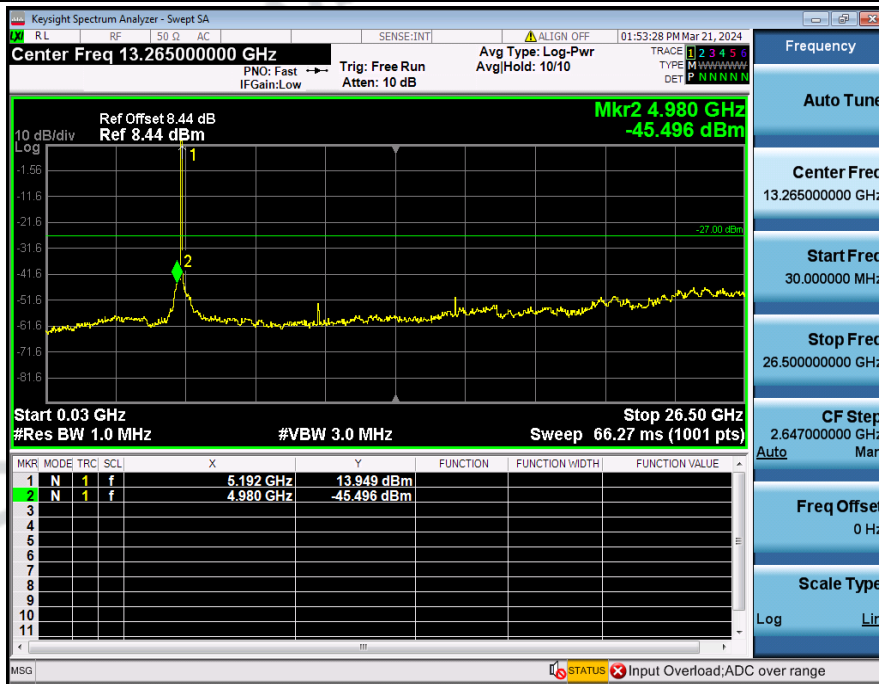
Spurious_Emission_NVNT_3TXx3RX_802_11ac(VHT20)_5180_20M
