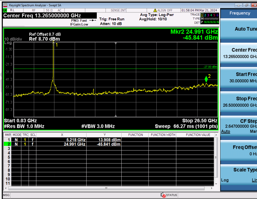
Spurious_Emission_NVNT_3TXx3RX_802_11ax(HE20)_5200_20M
