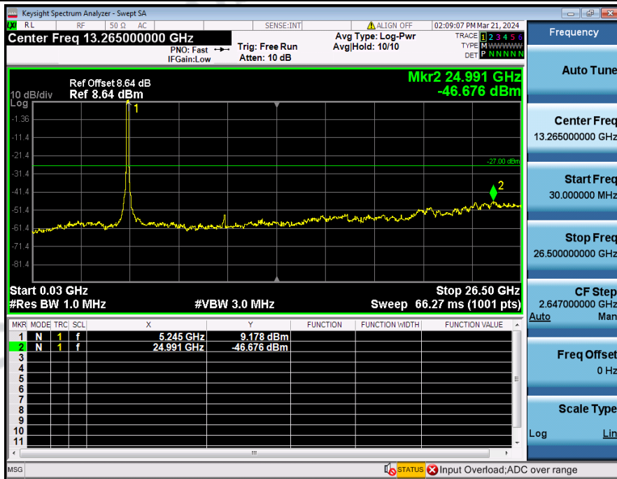
Spurious_Emission_NVNT_3TXx3RX_802_11ac(VHT80)_5210_80M
