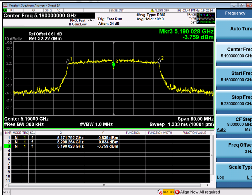
Frequency_Stability_NVNT_ANT3_802_11n(HT40)_5190
