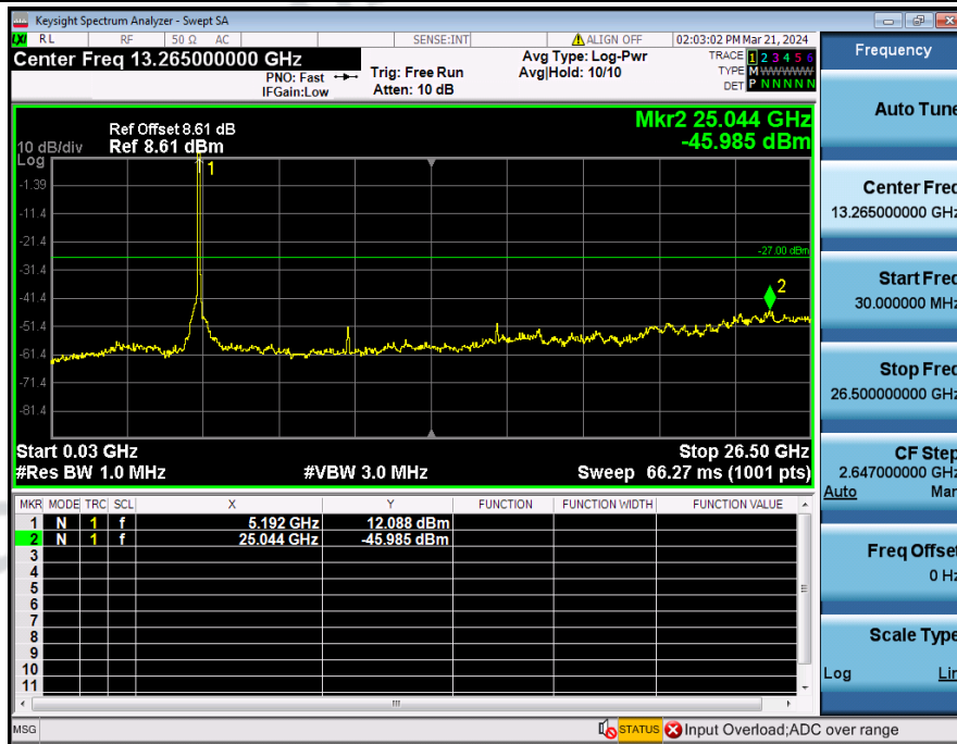
Spurious_Emission_NVNT_3TXx3RX_802_11ac(VHT40)_5190_40M
