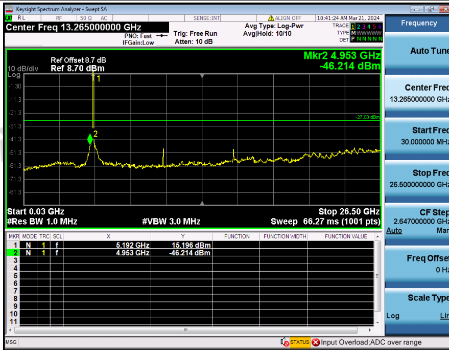
Spurious_Emission_NVNT_3TXx3RX_802_11a_5200_20M
