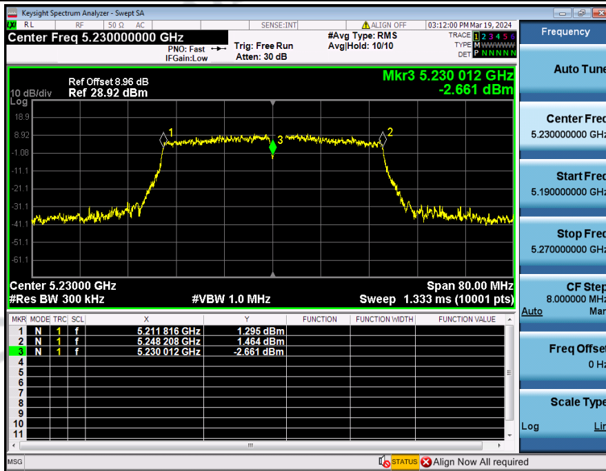
Frequency_Stability_NVNT_ANT3_802_11n(HT40)_5230
