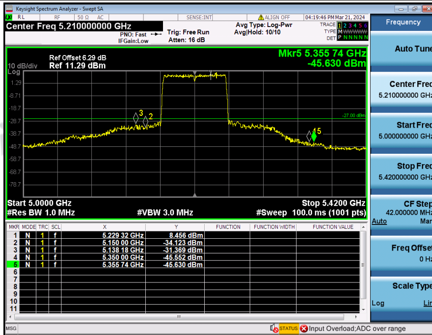
Bandedge_NVNT_ANT2_802_11ac(VHT80)_5210
