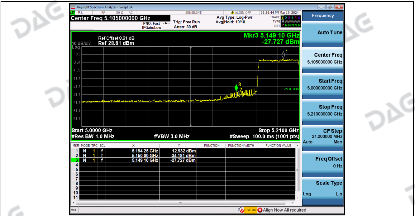
Bandedge_NVNT_ANT1_802_11ax(HE40)_5230
