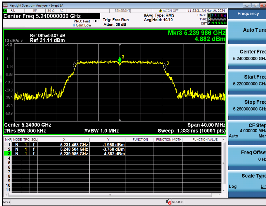
Frequency_Stability_NVNT_ANT2_802_11a_5240
