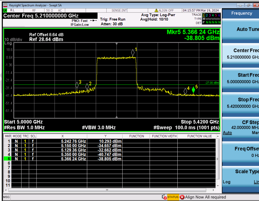
Bandedge_NVNT_ANT3_802_11ax(HE80)_5210
