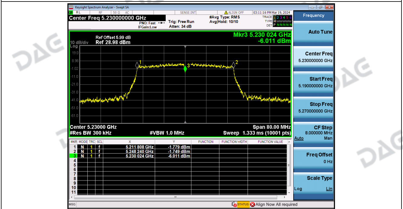
Frequency_Stability_NVNT_ANT2_802_11n(HT40)_5230
