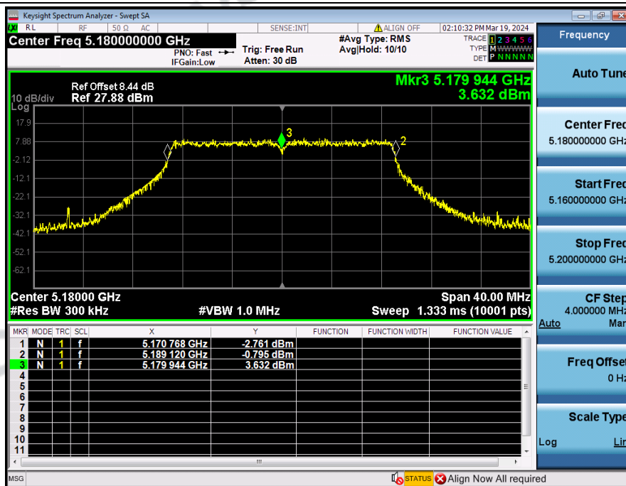
Frequency_Stability_NVNT_ANT3_802_11ac(VHT20)_5180
