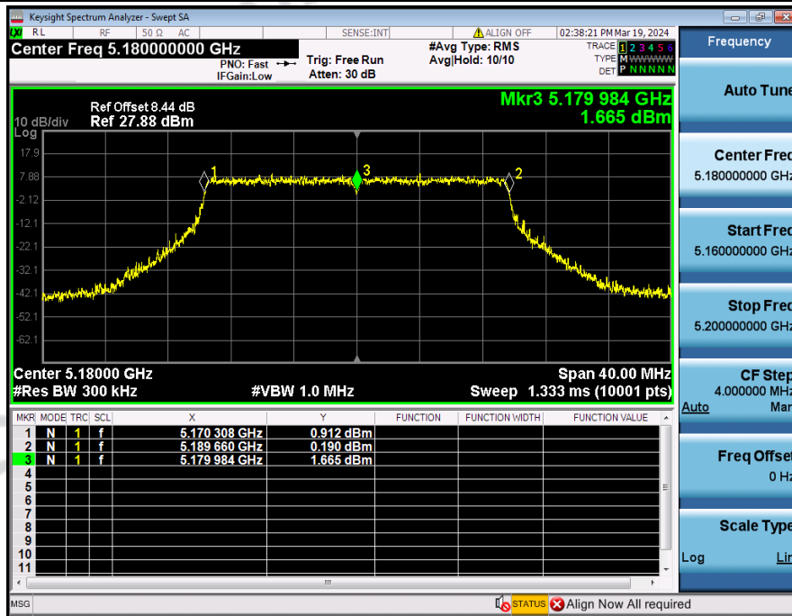
Frequency_Stability_NVNT_ANT3_802_11ax(HE20)_5180
