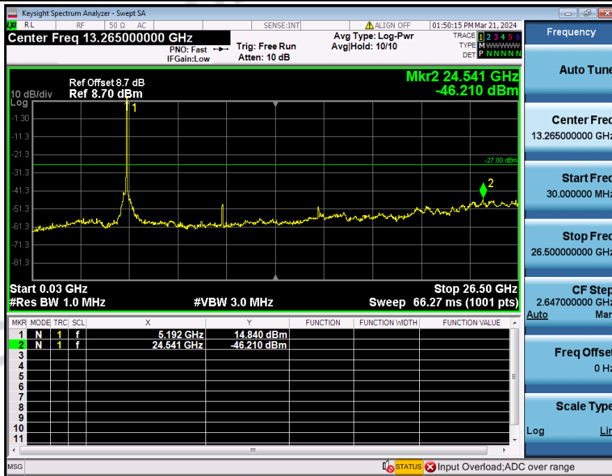
Spurious_Emission_NVNT_3TXx3RX_802_11n(HT20)_5200_20M
