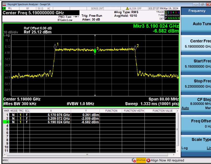
Frequency_Stability_NVNT_ANT2_802_11ax(HE40)_5190
