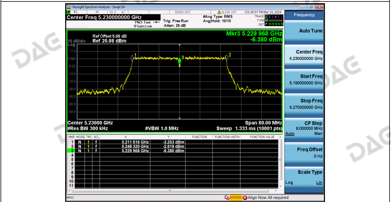
Frequency_Stability_NVNT_ANT2_802_11ac(VHT40)_5230
