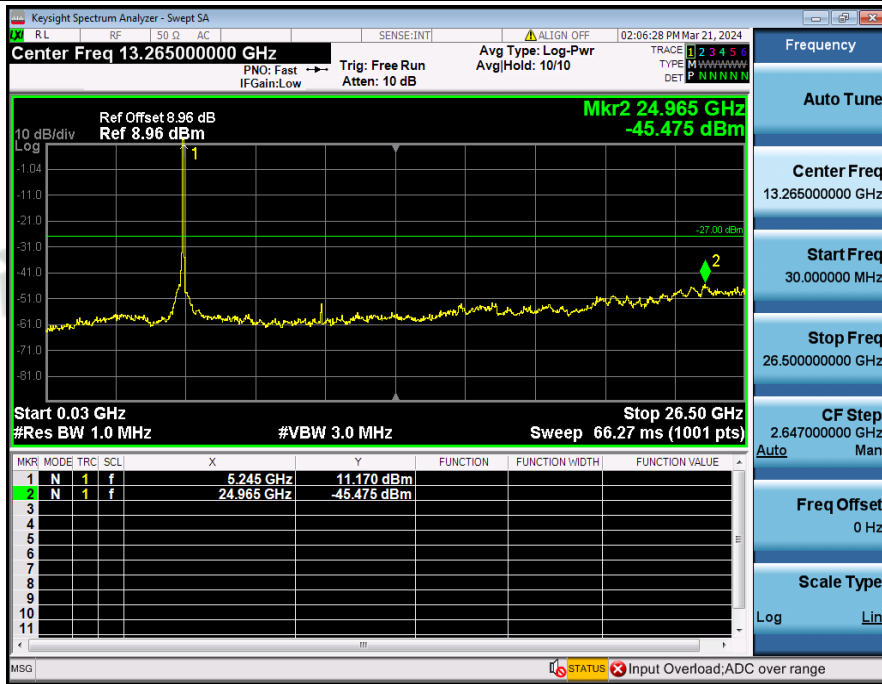
Spurious_Emission_NVNT_3TXx3RX_802_11ax(HE40)_5230_40M
