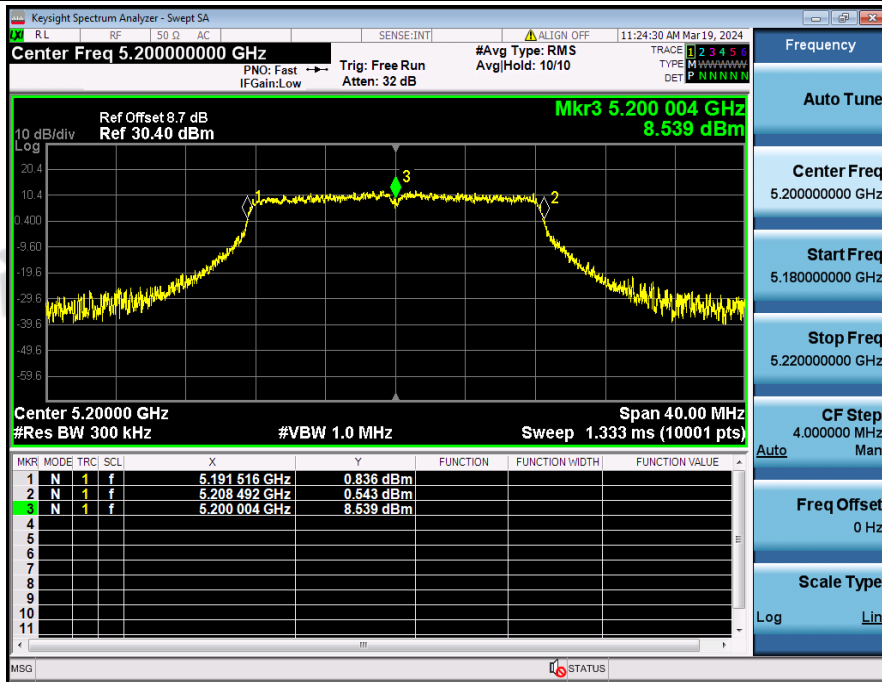
Frequency_Stability_NVNT_ANT3_802_11a_5200
