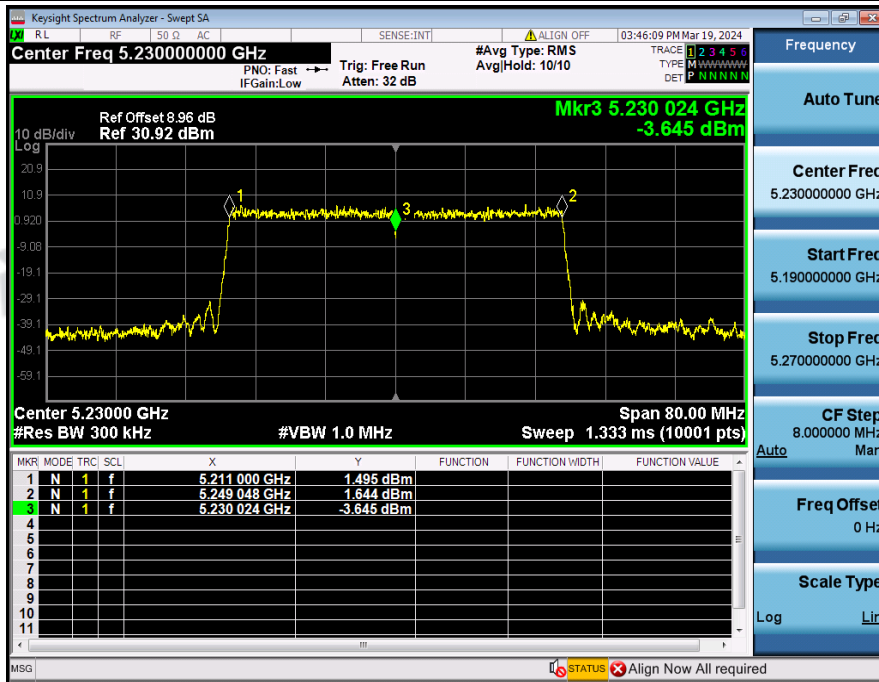
Frequency_Stability_NVNT_ANT3_802_11ax(HE40)_5230
