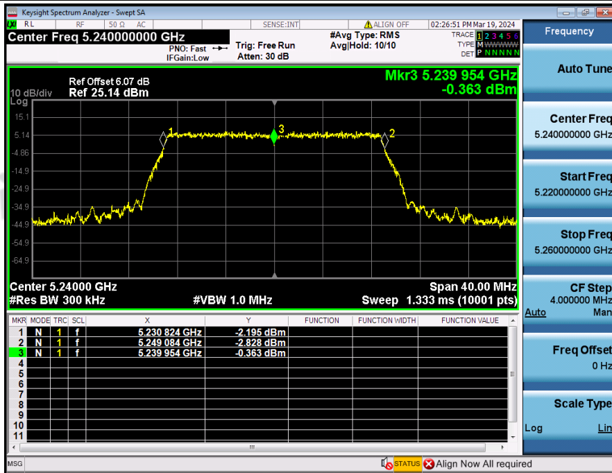
Frequency_Stability_NVNT_ANT2_802_11ac(VHT20)_5240
