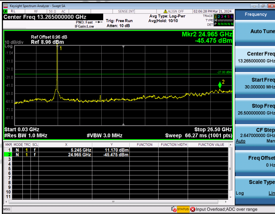
Spurious_Emission_NVNT_3TXx3RX_802_11ax(HE40)_5230_40M
