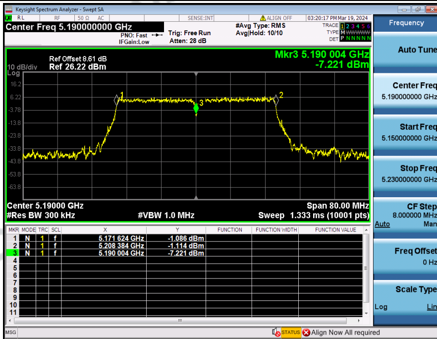
Frequency_Stability_NVNT_ANT3_802_11ac(VHT40)_5190
