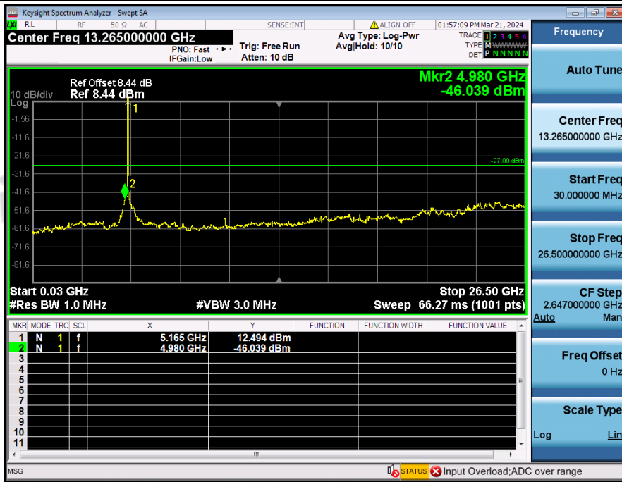
Spurious_Emission_NVNT_3TXx3RX_802_11ax(HE20)_5180_20M
