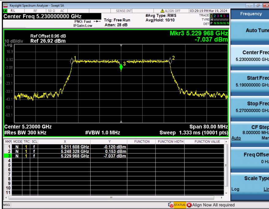
Frequency_Stability_NVNT_ANT3_802_11ac(VHT40)_5230
