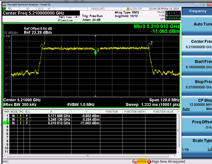
Frequency_Stability_NVNT_ANT3_802_11ac(VHT80)_5210
