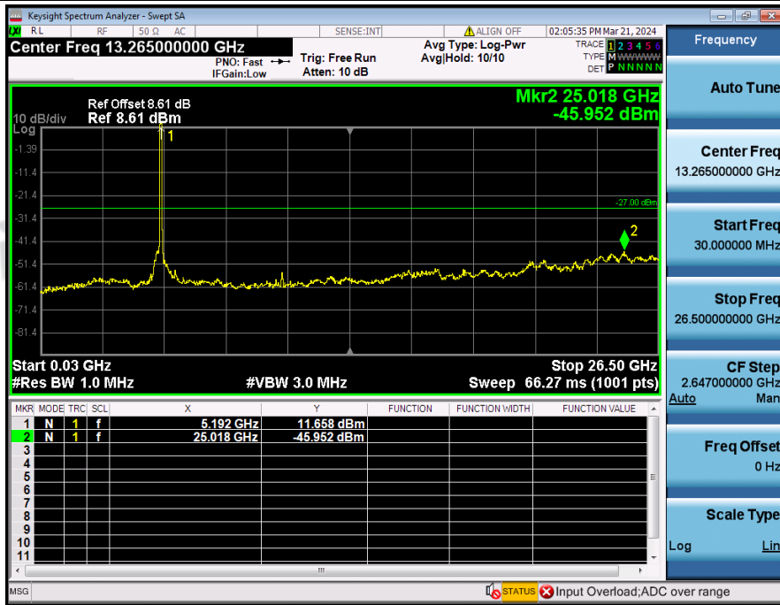
Spurious_Emission_NVNT_3TXx3RX_802_11ax(HE40)_5190_40M
