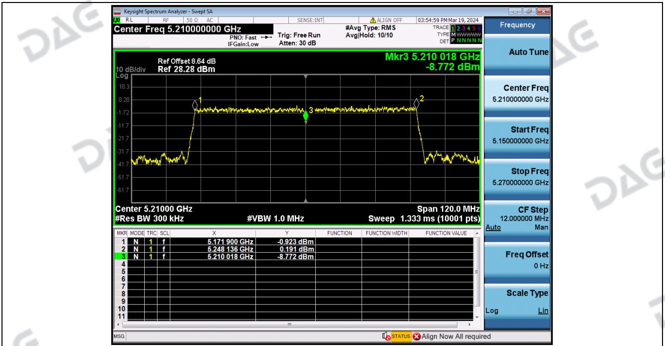
Frequency_Stability_NVNT_ANT1_802_11ax(HE80)_5210
