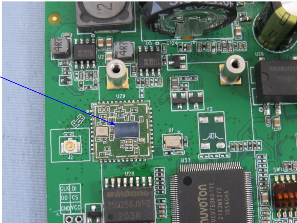
WIFI Chip
