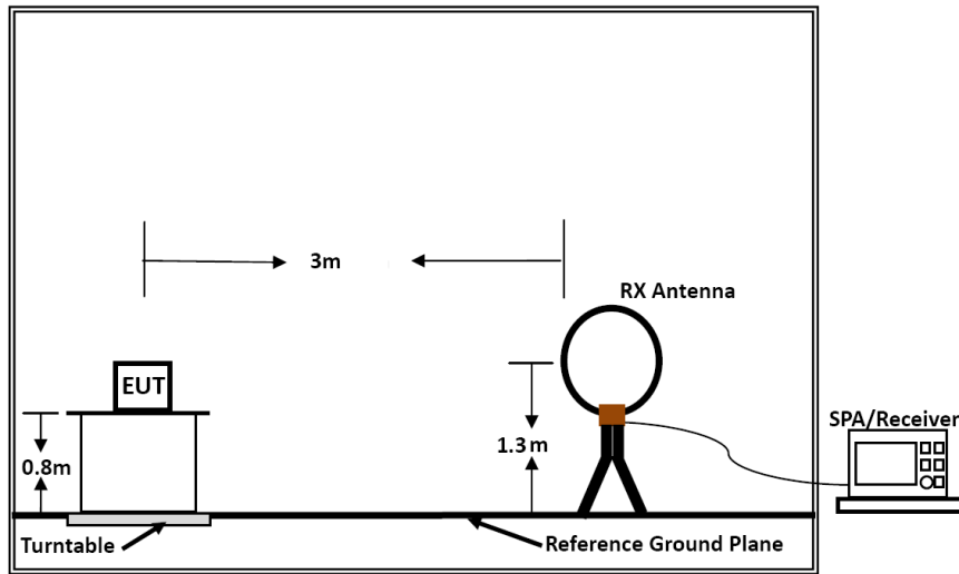
Below 30MHz
