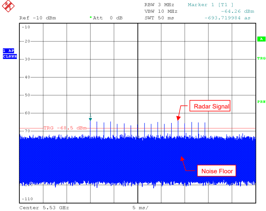
Radar Signal 0
