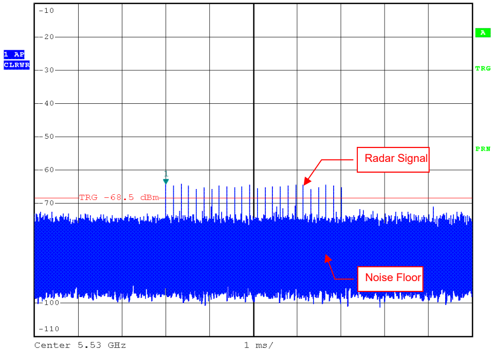
Radar Signal 2
