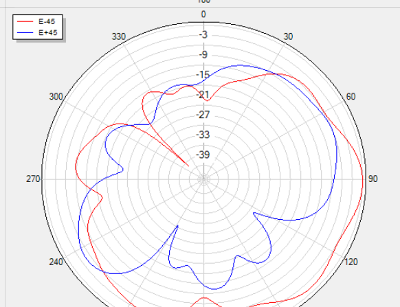
V Phi=0 freq=2410MHz
