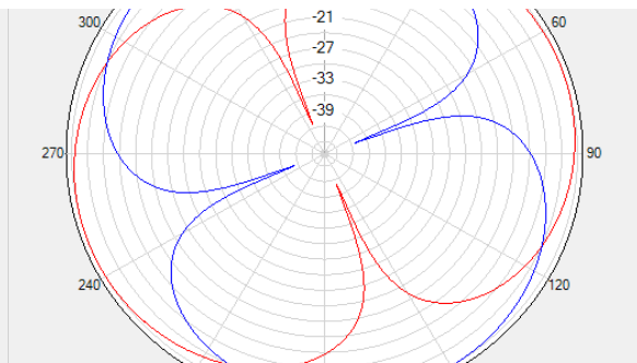
H Theta=0 freq=2600MHz
