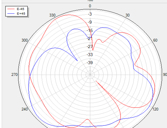
V Phi=90 freq=2410MHz
