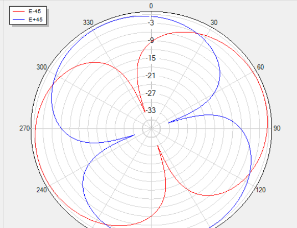
V Phi=0 freq=2400MHz
