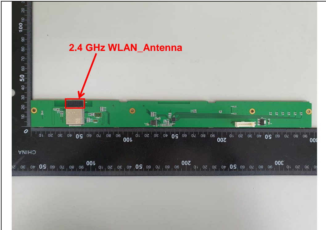
LED Board_Rear
