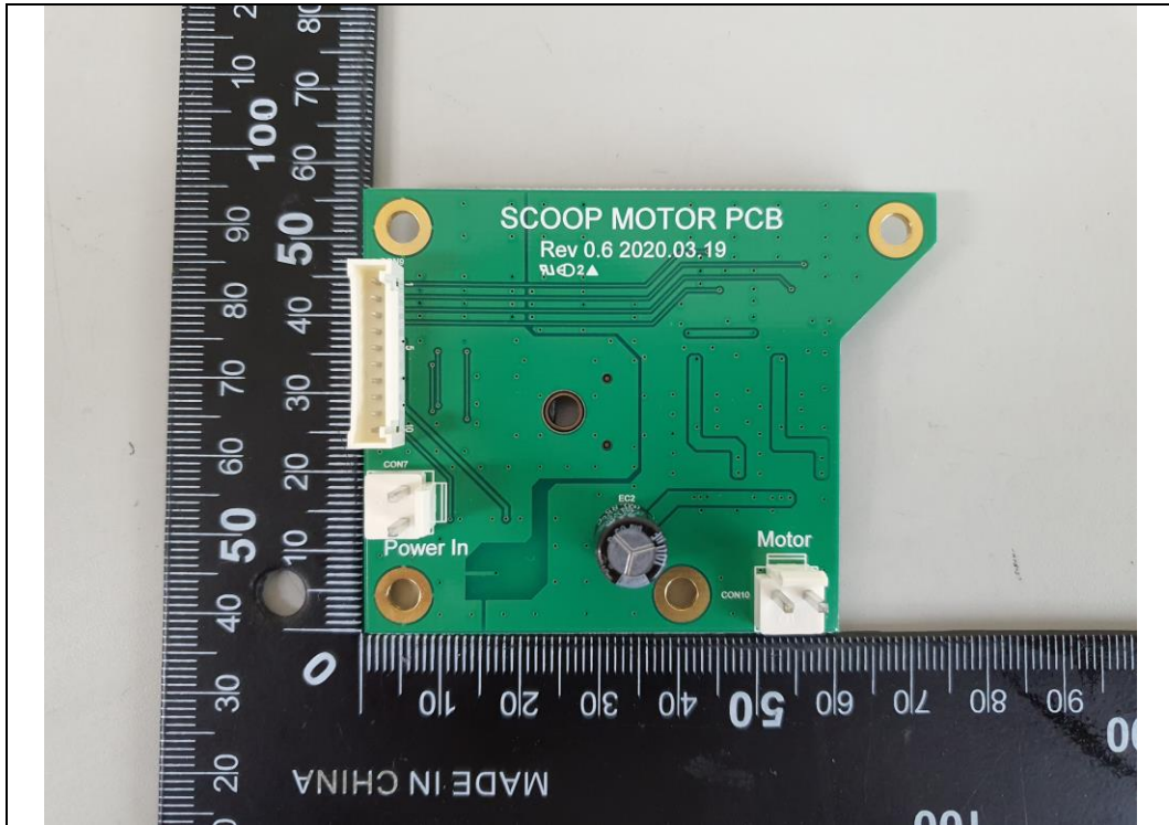
Motor Board Front
