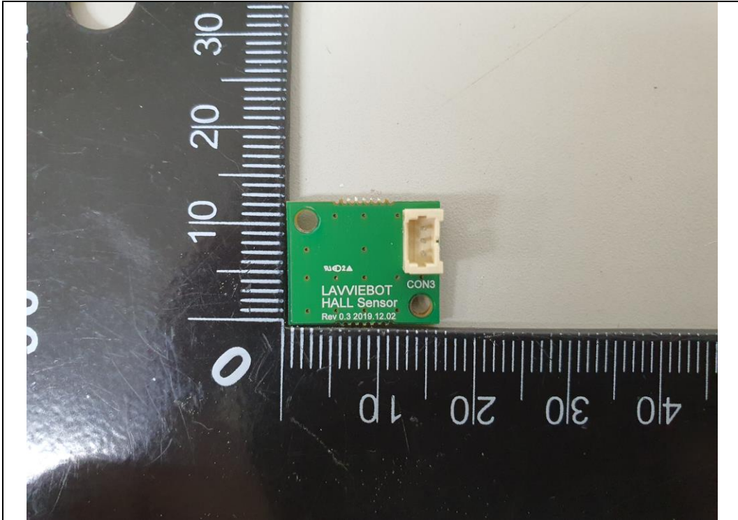
Hall Sensor Board_Front
