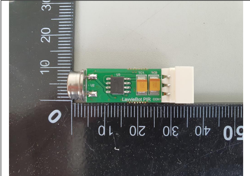
PIR Board Front
