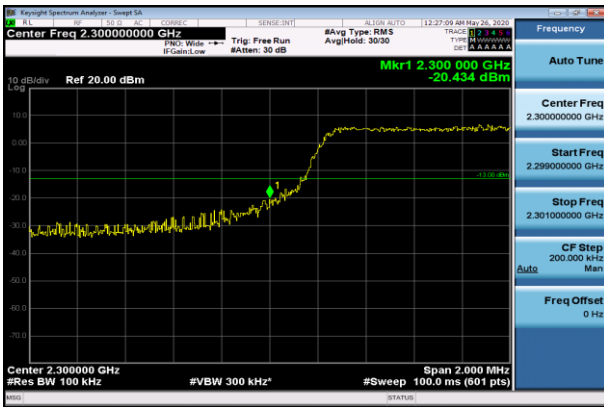
LCH_16QAM_25RB#0
