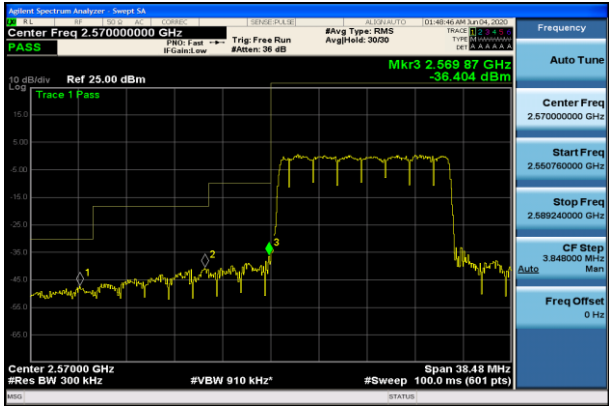
LCH_QPSK_75RB#0
