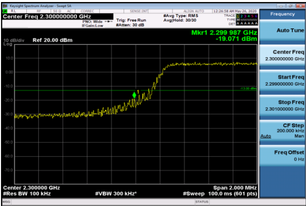
LCH_QPSK_25RB#0
