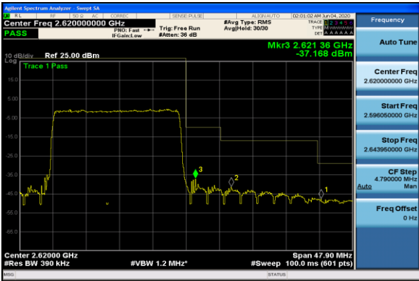
HCH_QPSK_100RB#0
