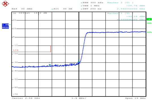
LCH_QPSK_100RB#0
