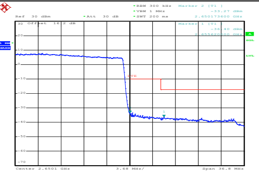
HCH_QPSK_100RB#0
