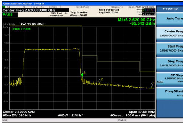
HCH_16QAM_100RB#0
