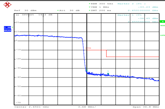
HCH_16QAM_100RB#0
