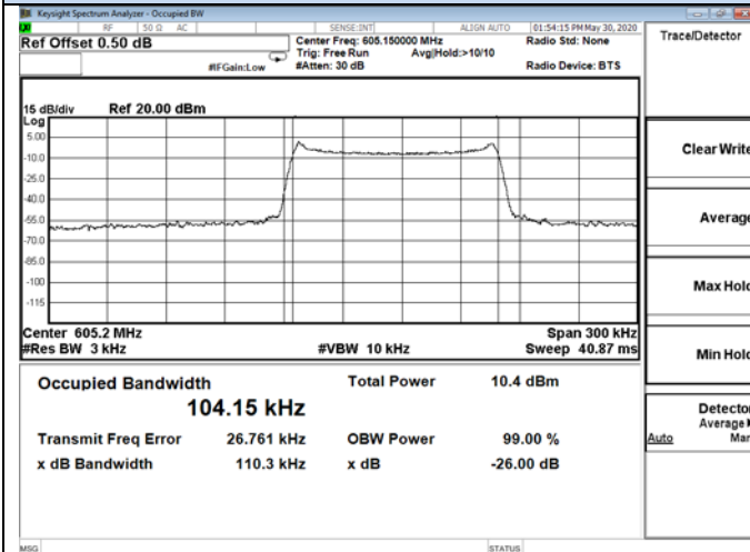
Channel 36 / 605.15 MHz
