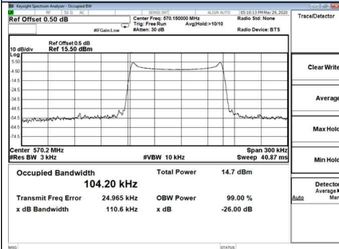
Channel 01 / 570.15 MHz
