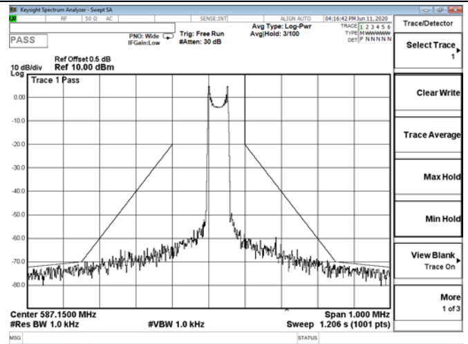
Channel 18 / 587.15 MHz
