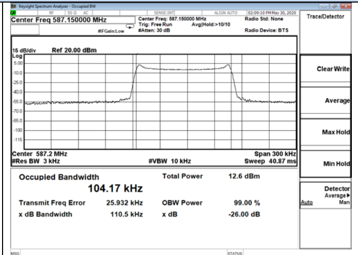
Channel 18 / 587.15 MHz
