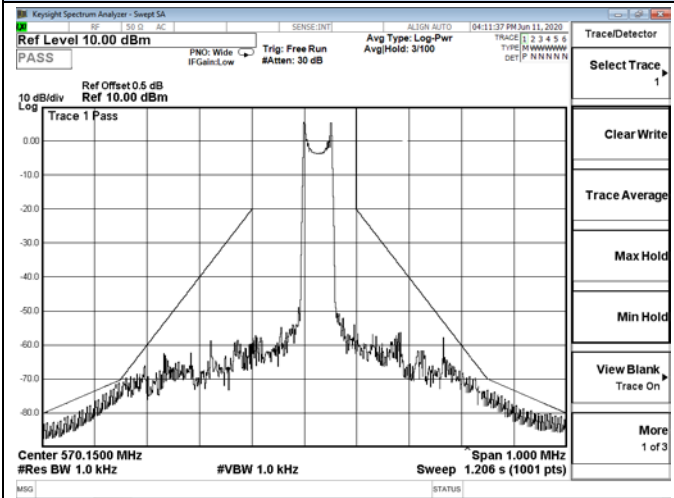
Channel 01 / 570.15 MHz
